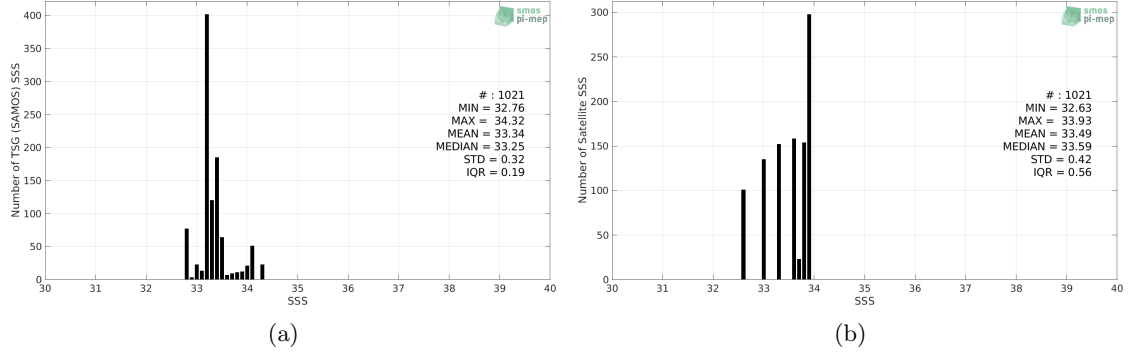
Figure 2: Histograms of SSS from TSG (SAMOS) (a) and Aquarius SSS L4 OI v5 - Weekly (IPRC) (b) considering all match-up pairs per bins of 0.1 over the Ganga and Brahmaputra river plumes Pi-MEP region and for the full satellite product period.
