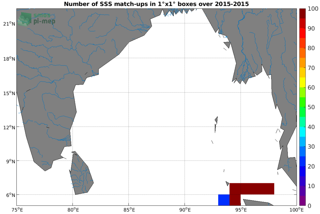
Figure 4: Number of SSS match-ups between TSG (SAMOS) SSS and the Aquarius SSS L4 OI v5 - Weekly (IPRC) SSS product for the Ganga and Brahmaputra river plumes Pi-MEP region over 1^\circ \times 1^\circ boxes and for the full satellite product period.
