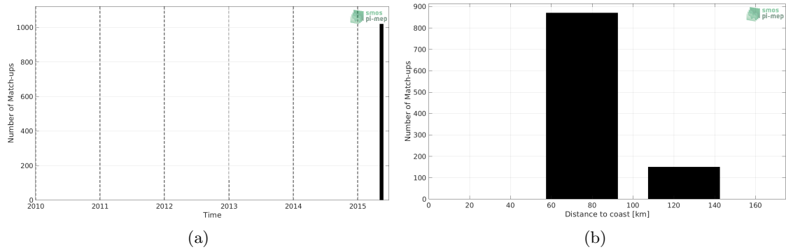
Figure 1: Number of match-ups between TSG (SAMOS) and Aquarius SSS L4 OI v5 - Weekly (IPRC) SSS as a function of time (a) and as function of the distance to coast (b) over the Ganga and Brahmaputra river plumes Pi-MEP region and for the full satellite product period.
