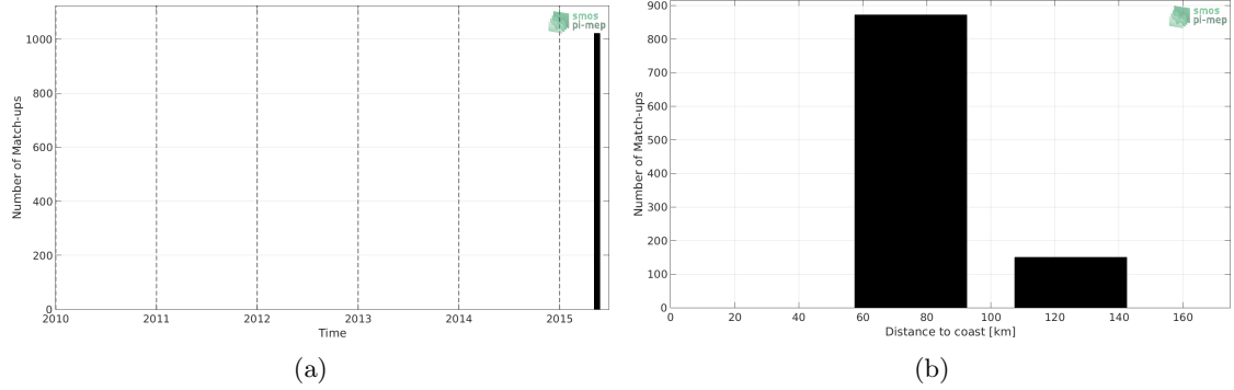
Figure 1: Number of match-ups between TSG-SAMOS and Aquarius-L4-IPRC-V5-WEEKLY SSS as a function of time (a) and as function of the distance to coast (b) over the Ganga and Brahmaputra river plumes Pi-MEP region and for the full satellite product period.
