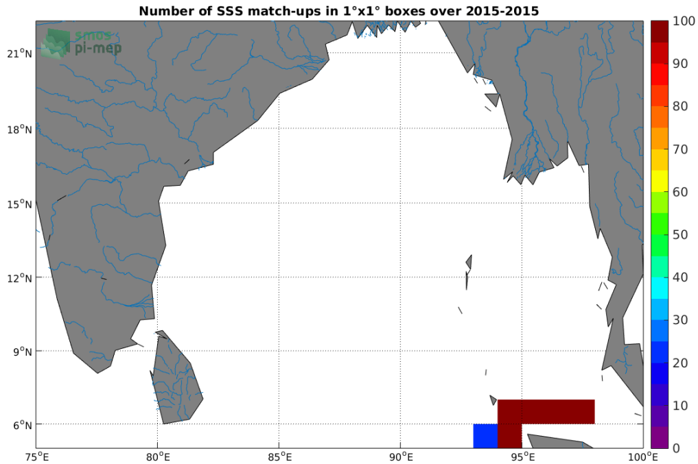
Figure 4: Number of SSS match-ups between TSG-SAMOS SSS and the Aquarius-L4-IPRC-V5-WEEKLY SSS product for the Ganga and Brahmaputra river plumes Pi-MEP region over 1°x1° boxes and for the full satellite product period.
