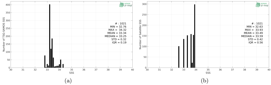
Figure 2: Histograms of SSS from TSG-SAMOS (a) and Aquarius-L4-IPRC-V5-WEEKLY (b) considering all match-up pairs per bins of 0.1 over the Ganga and Brahmaputra river plumes Pi-MEP region and for the full satellite product period.
