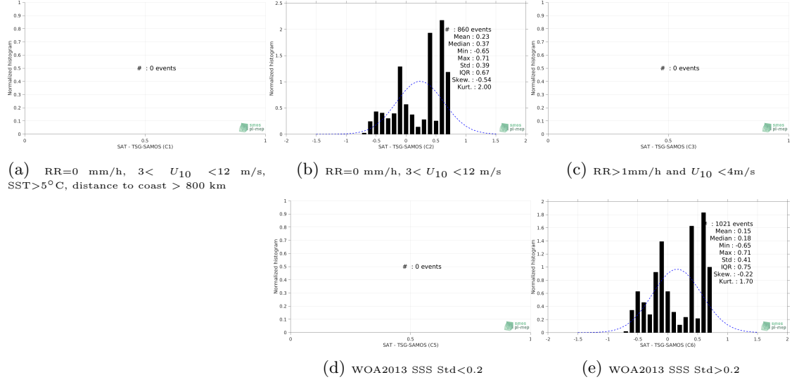
Figure 13: Normalized histogram of \Delta\text{SSS} (Aquarius-L4-IPRC-V5-WEEKLY - TSG-SAMOS) for 5 different subdatasets corresponding to: RR=0 mm/h, 3 < U_{10} < 12 m/s, SST > 5^\circ\text{C} , distance to coast > 800 km (a), RR=0 mm/h, 3 < U_{10} < 12 m/s (b), RR > 1 mm/h and U_{10} < 4 m/s (c), WOA2013 SSS Std < 0.2 (d), WOA2013 SSS Std > 0.2 (e).
