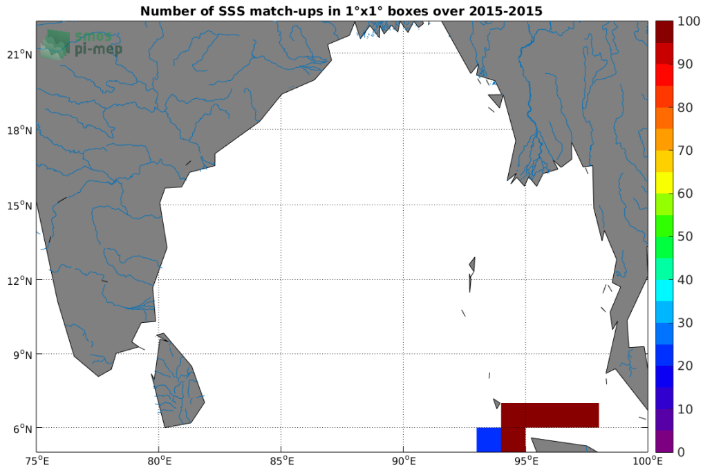
Figure 4: Number of SSS match-ups between TSG-SAMOS SSS and the Aquarius-L4-IPRC-V5-WEEKLY SSS product for the Ganga and Brahmaputra river plumes Pi-MEP region over 1^\circ \times 1^\circ boxes and for the full satellite product period.
