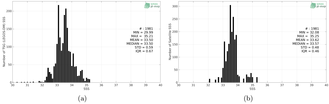
Figure 2: Histograms of SSS from TSG (LEGOS-DM) (a) and Aquarius SSS L4 OI v5 - Weekly (IPRC) (b) considering all match-up pairs per bins of 0.1 over the Ganga and Brahmaputra river plumes Pi-MEP region and for the full satellite product period.
