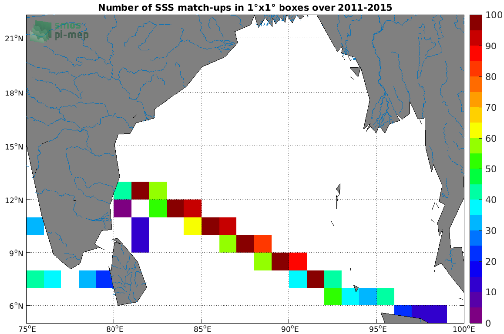
Figure 4: Number of SSS match-ups between TSG (LEGOS-DM) SSS and the Aquarius SSS L4 OI v5 - Weekly (IPRC) SSS product for the Ganga and Brahmaputra river plumes Pi-MEP region over 1°x1° boxes and for the full satellite product period.
