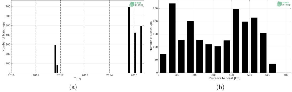
Figure 1: Number of match-ups between TSG (LEGOS-DM) and Aquarius SSS L4 OI v5 - Weekly (IPRC) SSS as a function of time (a) and as function of the distance to coast (b) over the Ganga and Brahmaputra river plumes Pi-MEP region and for the full satellite product period.
