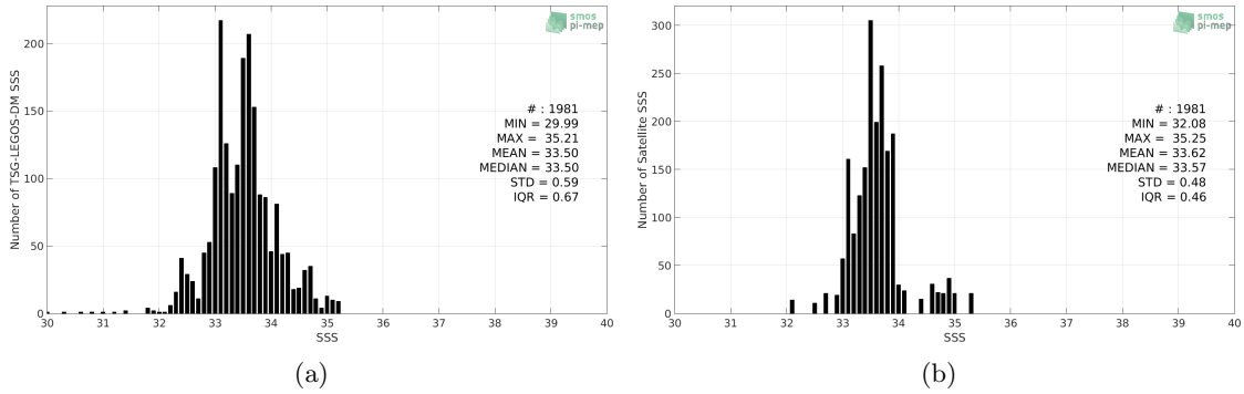
Figure 2: Histograms of SSS from TSG-LEGOS-DM (a) and Aquarius-L4-IPRC-V5-WEEKLY (b) considering all match-up pairs per bins of 0.1 over the Ganga and Brahmaputra river plumes Pi-MEP region and for the full satellite product period.
