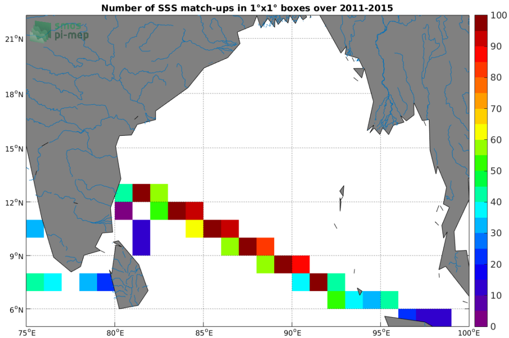
Figure 4: Number of SSS match-ups between TSG-LEGOS-DM SSS and the Aquarius-L4-IPRC-V5-WEEKLY SSS product for the Ganga and Brahmaputra river plumes Pi-MEP region over 1°x1° boxes and for the full satellite product period.
