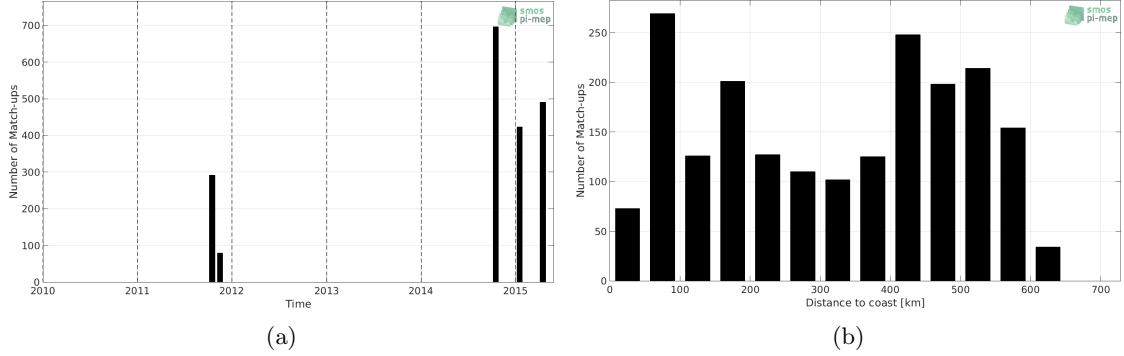
Figure 1: Number of match-ups between TSG-LEGOS-DM and Aquarius-L4-IPRC-V5-WEEKLY SSS as a function of time (a) and as function of the distance to coast (b) over the Ganga and Brahmaputra river plumes Pi-MEP region and for the full satellite product period.
