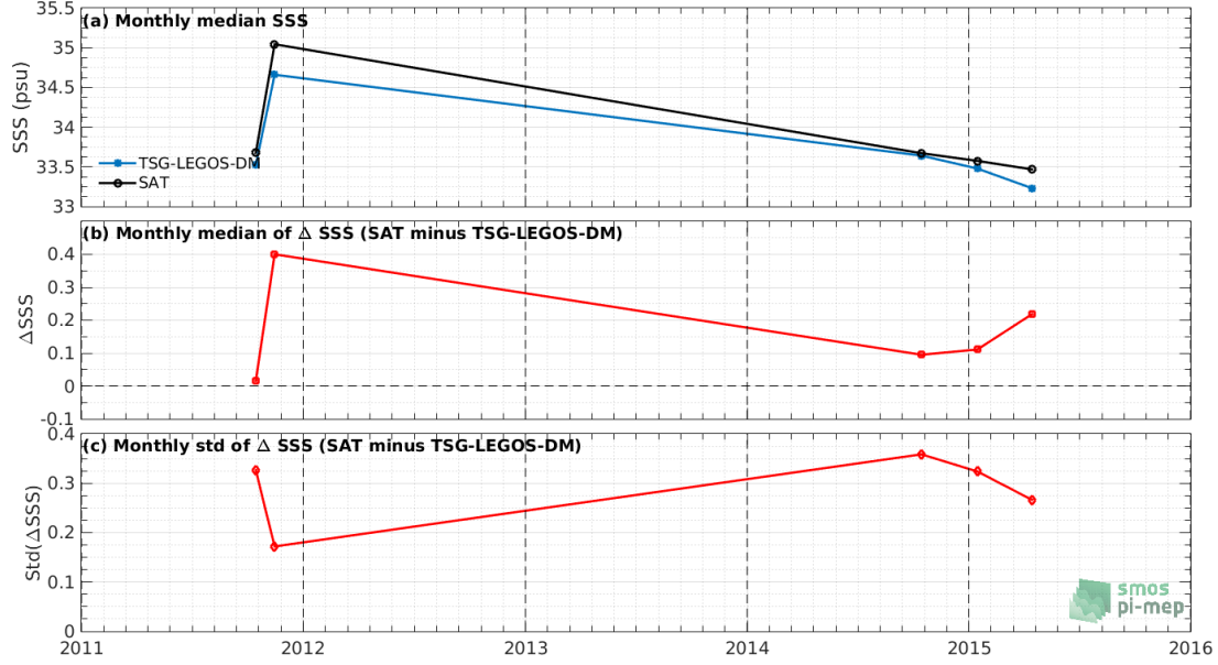
Figure 7: Time series of the monthly median SSS (top), median of \Delta\text{SSS} (Satellite - TSG-LEGOS-DM) and Std of \Delta\text{SSS} (Satellite - TSG-LEGOS-DM) over the Ganga and Brahmaputra river plumes Pi-MEP region considering all match-ups collected by the Pi-MEP.
