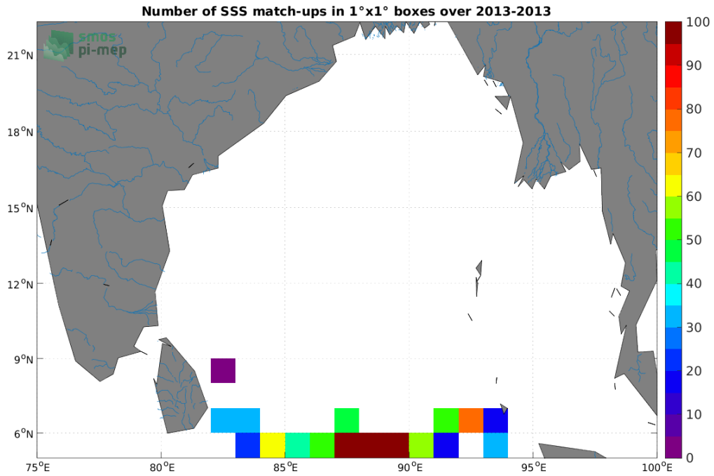
Figure 3: Number of SSS match-ups between Surface drifters SSS and the Aquarius SSS L4 OI v5 - Weekly (IPRC) SSS product for the Ganga and Brahmaputra river plumes Pi-MEP region over 1^\circ \times 1^\circ boxes and for the full satellite product period.
