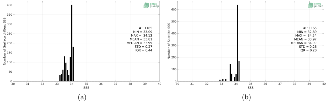
Figure 2: Histograms of SSS from Surface drifters (a) and Aquarius SSS L4 OI v5 - Weekly (IPRC) (b) considering all match-up pairs per bins of 0.1 over the Ganga and Brahmaputra river plumes Pi-MEP region and for the full satellite product period.
