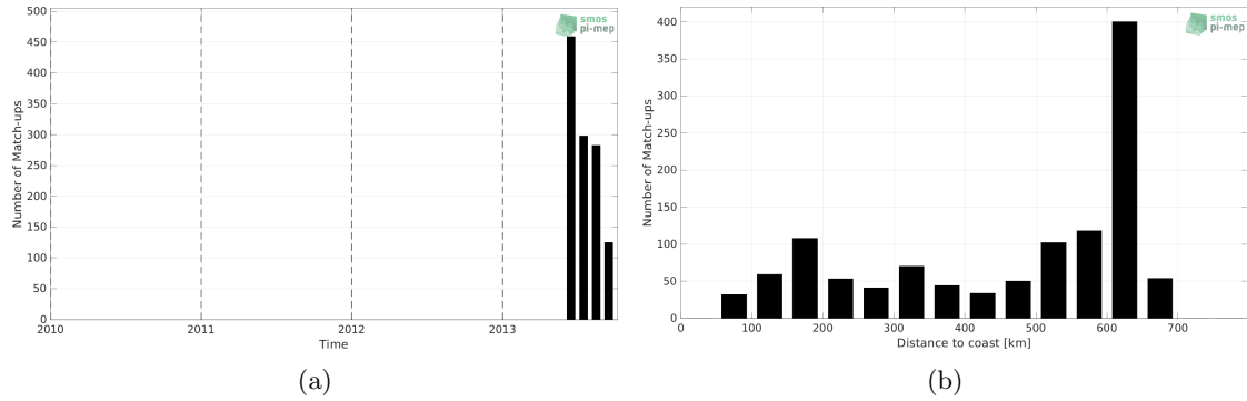
Figure 1: Number of match-ups between Surface drifters and Aquarius SSS L4 OI v5 - Weekly (IPRC) SSS as a function of time (a) and as function of the distance to coast (b) over the Ganga and Brahmaputra river plumes Pi-MEP region and for the full satellite product period.
