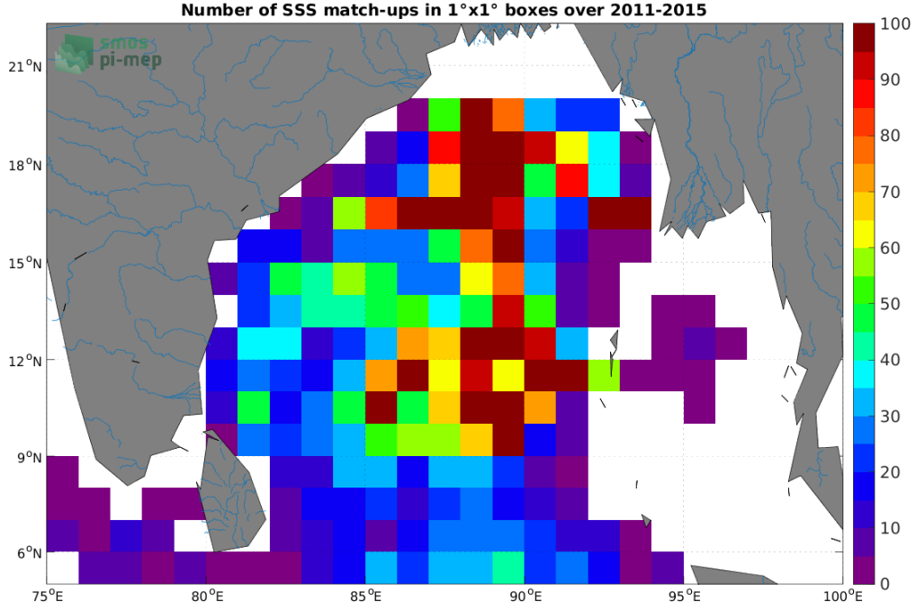
Figure 4: Number of SSS match-ups between Argo SSS and the Aquarius SSS L4 OI v5 - Weekly (IPRC) SSS product for the Ganga and Brahmaputra river plumes Pi-MEP region over 1°x1° boxes and for the full satellite product period.
