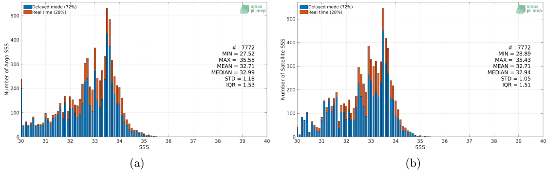
Figure 2: Histograms of SSS from Argo (a) and Aquarius SSS L4 OI v5 - Weekly (IPRC) (b) considering all match-up pairs per bins of 0.1 over the Ganga and Brahmaputra river plumes Pi-MEP region and for the full satellite product period.
