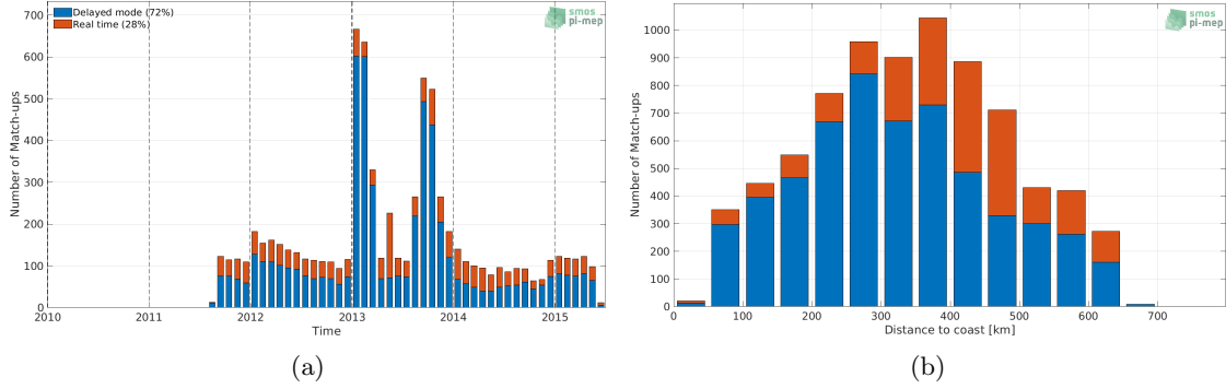
Figure 1: Number of match-ups between Argo and Aquarius SSS L4 OI v5 - Weekly (IPRC) SSS as a function of time (a) and as function of the distance to coast (b) over the Ganga and Brahmaputra river plumes Pi-MEP region and for the full satellite product period.
