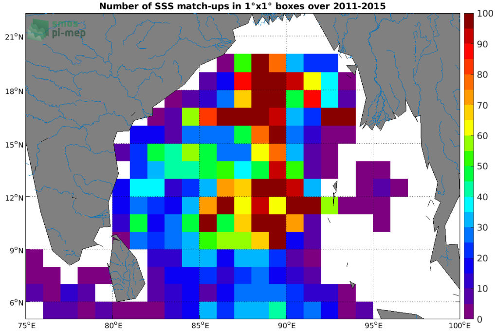
Figure 4: Number of SSS match-ups between Argo SSS and the Aquarius SSS L4 OI v5 - Weekly (IPRC) SSS product for the Ganga and Brahmaputra river plumes Pi-MEP region over 1^\circ \times 1^\circ boxes and for the full satellite product period.
