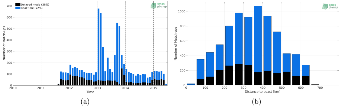
Figure 1: Number of match-ups between Argo and Aquarius-L4-IPRC-V5-WEEKLY SSS as a function of time (a) and as function of the distance to coast (b) over the Ganga and Brahmaputra river plumes Pi-MEP region and for the full satellite product period.
