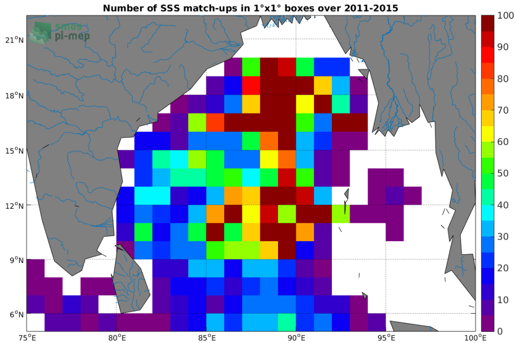
Figure 4: Number of SSS match-ups between Argo SSS and the Aquarius-L4-IPRC-V5-WEEKLY SSS product for the Ganga and Brahmaputra river plumes Pi-MEP region over 1°x1° boxes and for the full satellite product period.
