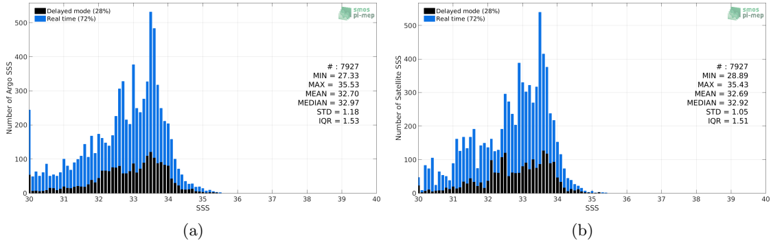
Figure 2: Histograms of SSS from Argo (a) and Aquarius-L4-IPRC-V5-WEEKLY (b) considering all match-up pairs per bins of 0.1 over the Ganga and Brahmaputra river plumes Pi-MEP region and for the full satellite product period.
