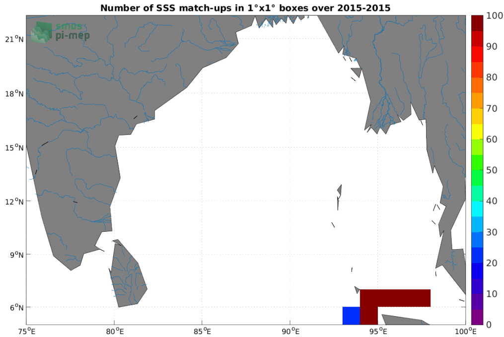
Figure 4: Number of SSS match-ups between TSG (SAMOS) SSS and the Aquarius SSS L4 OI v5 - Monthly (IPRC) SSS product for the Ganga and Brahmaputra river plumes Pi-MEP region over 1°×1° boxes and for the full satellite product period.
