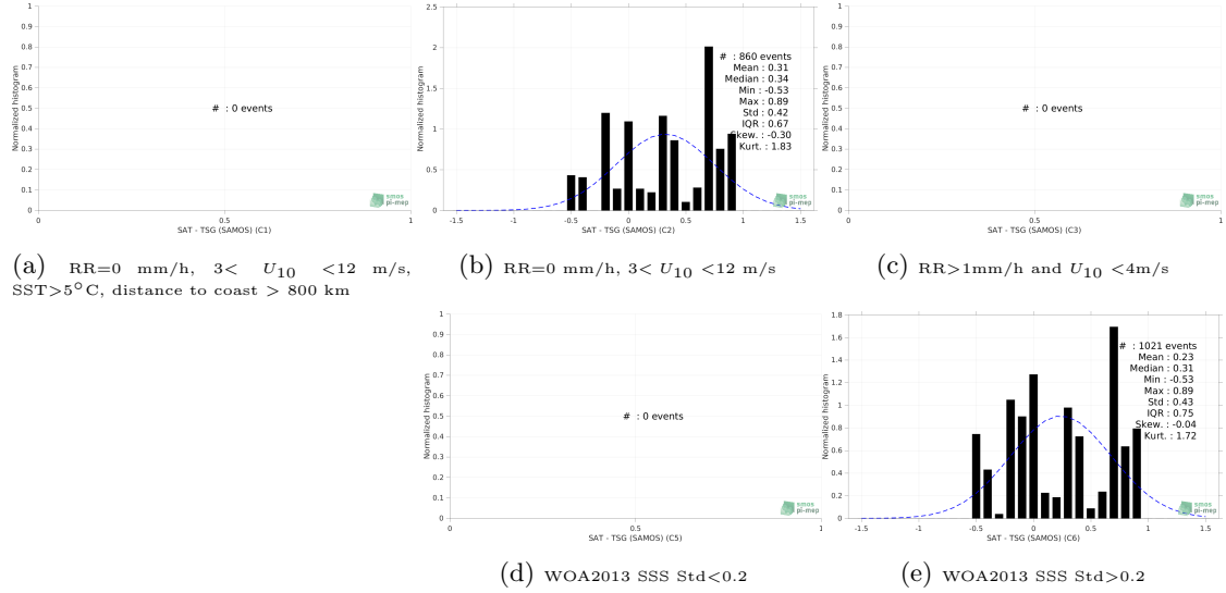
Figure 13: Normalized histogram of \Delta SSS (Aquarius SSS L4 OI v5 - Monthly (IPRC) - TSG (SAMOS)) for 5 different subdatasets corresponding to: RR=0 mm/h, 3 < U_{10} < 12 m/s, SST >5^{\circ} C, distance to coast > 800 km (a), RR=0 mm/h, 3 < U_{10} < 12 m/s (b), RR >1 mm/h and U_{10} < 4 m/s (c), WOA2013 SSS Std <0.2 (d), WOA2013 SSS Std >0.2 (e).
