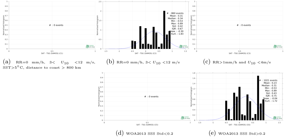
Figure 13: Normalized histogram of \Delta SSS (Aquarius SSS L4 OI v5 - Monthly (IPRC) - TSG (SAMOS)) for 5 different subdatasets corresponding to: RR=0 mm/h, 3 < U_{10} < 12 m/s, SST >5^{\circ} C, distance to coast > 800 km (a), RR=0 mm/h, 3 < U_{10} < 12 m/s (b), RR >1 mm/h and U_{10} < 4 m/s (c), WOA2013 SSS Std <0.2 (d), WOA2013 SSS Std >0.2 (e).
