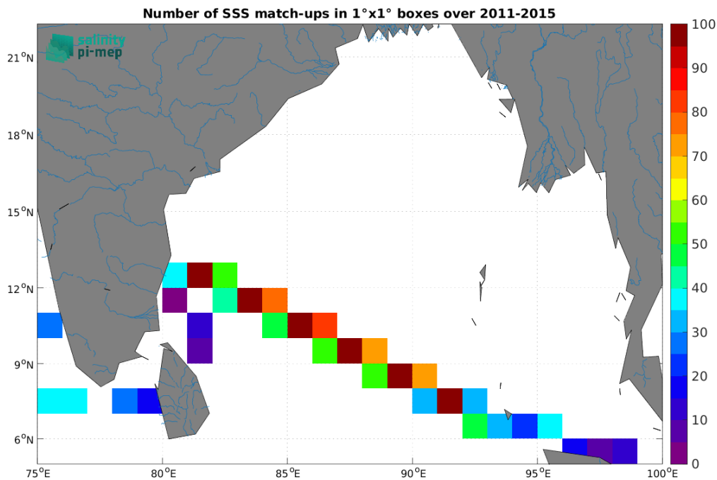
Figure 5: Number of SSS match-ups between TSG (LEGOS-DM) SSS and the Aquarius SSS L4 OI v5 - Monthly (IPRC) SSS product for the Ganga and Brahmaputra river plumes Pi-MEP region over 1^\circ \times 1^\circ boxes and for the full satellite product period.
