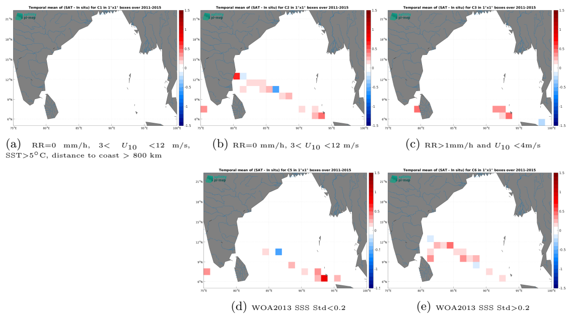
Figure 14: Temporal mean gridded over spatial boxes of size 1^\circ \times 1^\circ of \Delta SSS (Aquarius SSS L4 OI v5 - Monthly (IPRC) - TSG (LEGOS-DM)) for 5 different subdatasets corresponding to:RR=0 mm/h, 3 < U_{10} < 12 m/s, SST >5^\circ C, distance to coast > 800 km (a), RR=0 mm/h, 3 < U_{10} < 12 m/s (b), RR >1 mm/h and U_{10} < 4 m/s (c), WOA2013 SSS Std <0.2 (d), WOA2013 SSS Std >0.2 (e).
