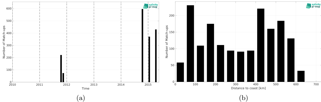
Figure 2: Number of match-ups between TSG (LEGOS-DM) and Aquarius SSS L4 OI v5 - Monthly (IPRC) SSS as a function of time (a) and as function of the distance to coast (b) over the Ganga and Brahmaputra river plumes Pi-MEP region and for the full satellite product period.
