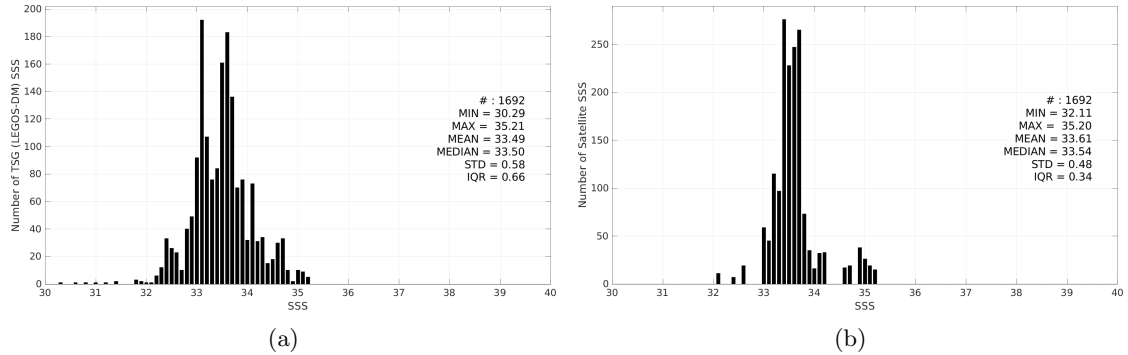
Figure 3: Histograms of SSS from TSG (LEGOS-DM) (a) and Aquarius SSS L4 OI v5 - Monthly (IPRC) (b) considering all match-up pairs per bins of 0.1 over the Ganga and Brahmaputra river plumes Pi-MEP region and for the full satellite product period.
