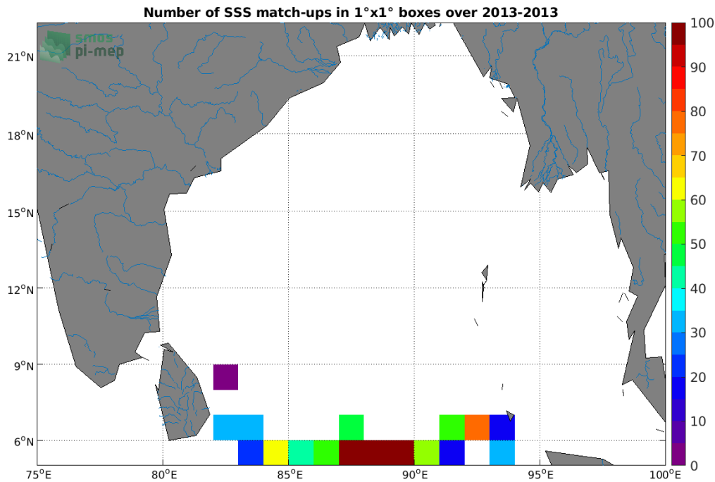
Figure 3: Number of SSS match-ups between Surface drifters SSS and the Aquarius SSS L4 OI v5 - Monthly (IPRC) SSS product for the Ganga and Brahmaputra river plumes Pi-MEP region over 1^\circ \times 1^\circ boxes and for the full satellite product period.
