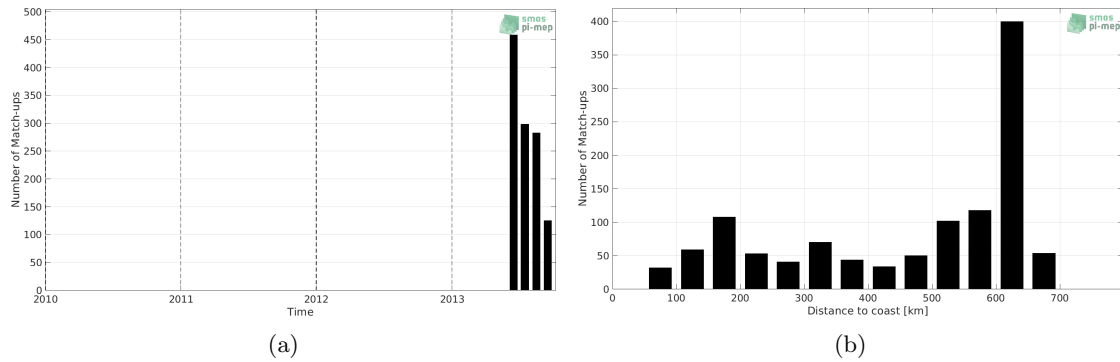
Figure 1: Number of match-ups between Surface drifters and Aquarius SSS L4 OI v5 - Monthly (IPRC) SSS as a function of time (a) and as function of the distance to coast (b) over the Ganga and Brahmaputra river plumes Pi-MEP region and for the full satellite product period.
