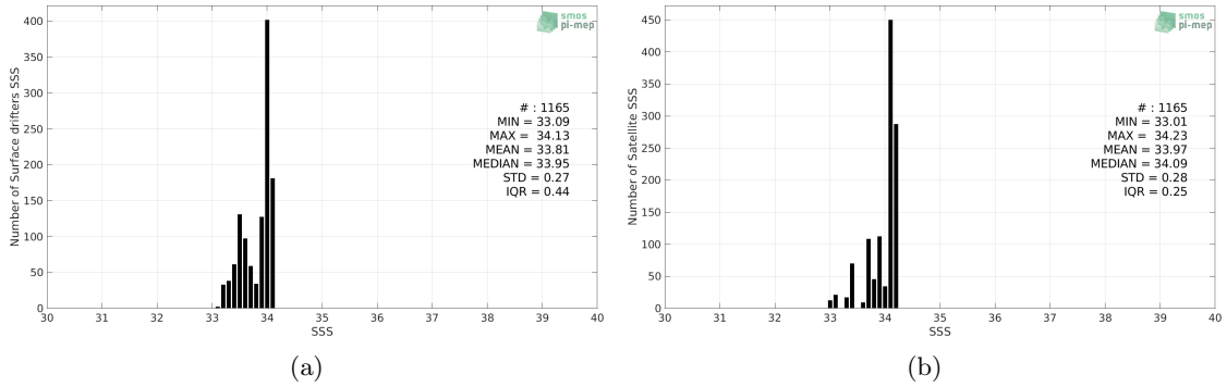
Figure 2: Histograms of SSS from Surface drifters (a) and Aquarius SSS L4 OI v5 - Monthly (IPRC) (b) considering all match-up pairs per bins of 0.1 over the Ganga and Brahmaputra river plumes Pi-MEP region and for the full satellite product period.
