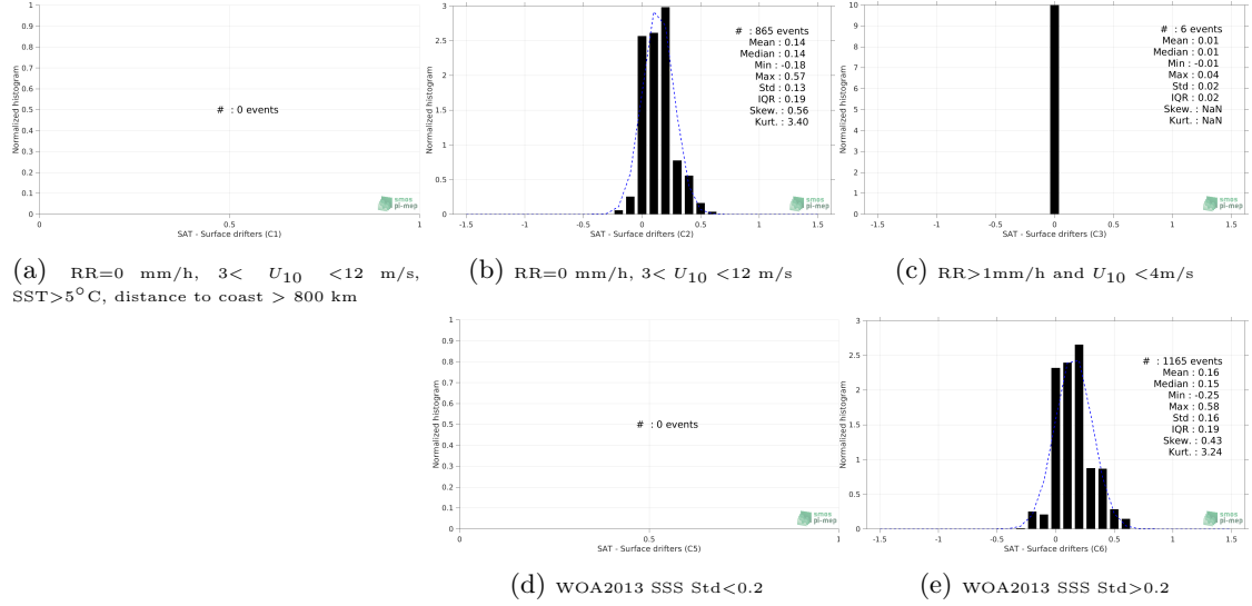
Figure 12: Normalized histogram of \Delta\text{SSS} (Aquarius SSS L4 OI v5 - Monthly (IPRC) - Surface drifters) for 5 different subdatasets corresponding to: RR=0 mm/h, 3 < U_{10} < 12 m/s, SST > 5^\circ\text{C} , distance to coast > 800 km (a), RR=0 mm/h, 3 < U_{10} < 12 m/s (b), RR > 1\text{mm/h} and U_{10} < 4\text{m/s} (c), WOA2013 SSS Std < 0.2 (d), WOA2013 SSS Std > 0.2 (e).
