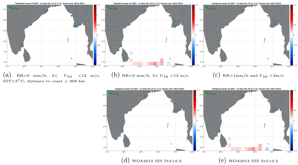
Figure 11: Temporal mean gridded over spatial boxes of size 1^\circ \times 1^\circ of \Delta SSS (Aquarius-L4-IPRC-V5-MONTHLY - Surface drifters) for 5 different subdatasets corresponding to:RR=0 mm/h, 3 < U_{10} < 12 m/s, SST >5^\circ C, distance to coast > 800 km (a), RR=0 mm/h, 3 < U_{10} < 12 m/s (b), RR >1 mm/h and U_{10} < 4 m/s (c), WOA2013 SSS Std <0.2 (d), WOA2013 SSS Std >0.2 (e).
