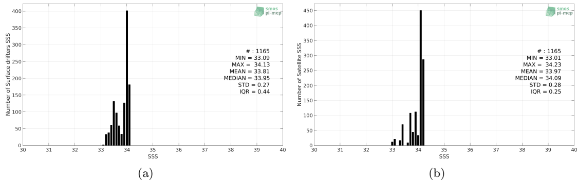
Figure 2: Histograms of SSS from Surface drifters (a) and Aquarius-L4-IPRC-V5-MONTHLY (b) considering all match-up pairs per bins of 0.1 over the Ganga and Brahmaputra river plumes Pi-MEP region and for the full satellite product period.
