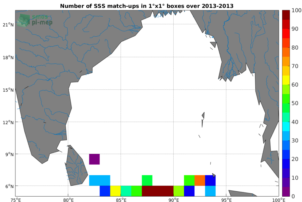
Figure 3: Number of SSS match-ups between Surface drifters SSS and the Aquarius-L4-IPRC-V5-MONTHLY SSS product for the Ganga and Brahmaputra river plumes Pi-MEP region over 1°x1° boxes and for the full satellite product period.
