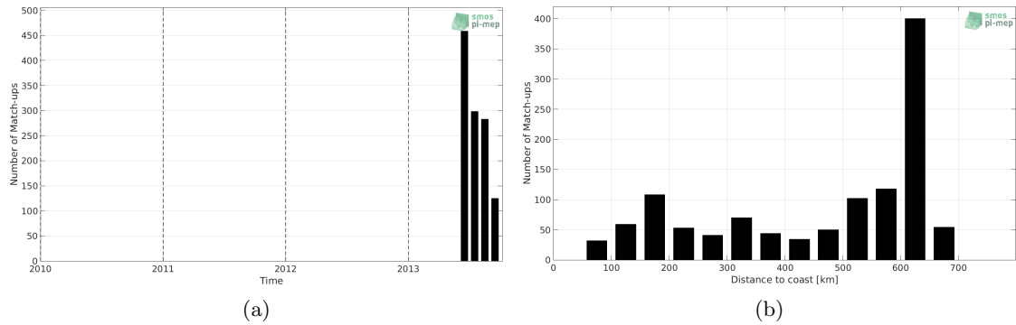
Figure 1: Number of match-ups between Surface drifters and Aquarius-L4-IPRC-V5-MONTHLY SSS as a function of time (a) and as function of the distance to coast (b) over the Ganga and Brahmaputra river plumes Pi-MEP region and for the full satellite product period.
