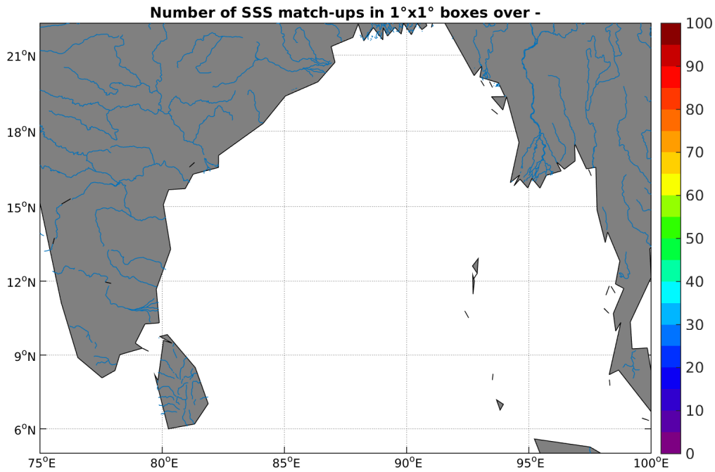
Figure 4: Number of SSS match-ups between TSG-GOSUD-Sailing-ship SSS and the Aquarius-L4-IPRC-V4-WEEKLY SSS product for the Ganga and Brahmaputra river plumes Pi-MEP region over 1°x1° boxes and for the full satellite product period.
