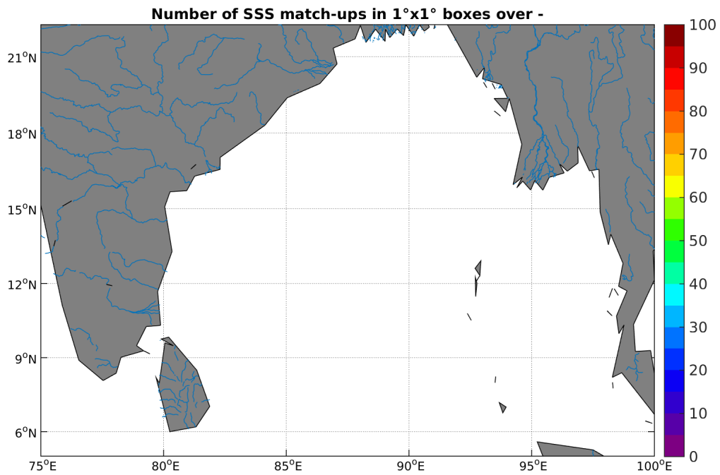
Figure 4: Number of SSS match-ups between TSG-GOSUD-Research-vessel SSS and the Aquarius-L4-IPRC-V4-WEEKLY SSS product for the Ganga and Brahmaputra river plumes Pi-MEP region over 1°x1° boxes and for the full satellite product period.
