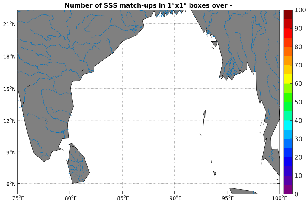
Figure 4: Number of SSS match-ups between Sea mammals SSS and the Aquarius-L4-IPRC-V4-WEEKLY SSS product for the Ganga and Brahmaputra river plumes Pi-MEP region over 1^\circ \times 1^\circ boxes and for the full satellite product period.
