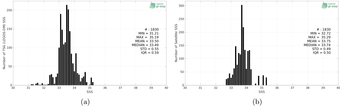
Figure 2: Histograms of SSS from TSG (LEGOS-DM) (a) and Aquarius SSS L3 CAP v5 - 7-Day running (JPL) (b) considering all match-up pairs per bins of 0.1 over the Ganga and Brahmaputra river plumes Pi-MEP region and for the full satellite product period.
