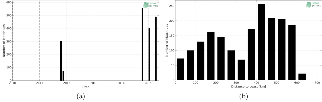
Figure 1: Number of match-ups between TSG (LEGOS-DM) and Aquarius SSS L3 CAP v5 - 7-Day running (JPL) SSS as a function of time (a) and as function of the distance to coast (b) over the Ganga and Brahmaputra river plumes Pi-MEP region and for the full satellite product period.
