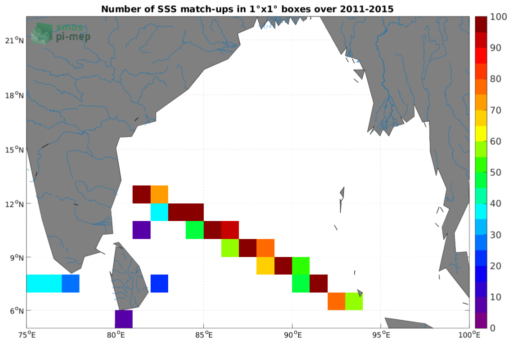
Figure 4: Number of SSS match-ups between TSG (LEGOS-DM) SSS and the Aquarius SSS L3 CAP v5 - 7-Day running (JPL) SSS product for the Ganga and Brahmaputra river plumes Pi-MEP region over 1^\circ \times 1^\circ boxes and for the full satellite product period.
