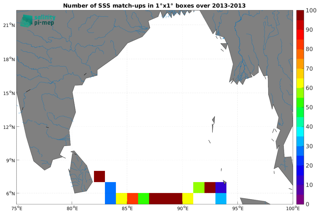
Figure 3: Number of SSS match-ups between Surface drifters SSS and the Aquarius SSS L3 CAP v5 - 7-Day running (JPL) SSS product for the Ganga and Brahmaputra river plumes Pi-MEP region over 1°×1° boxes and for the full satellite product period.
