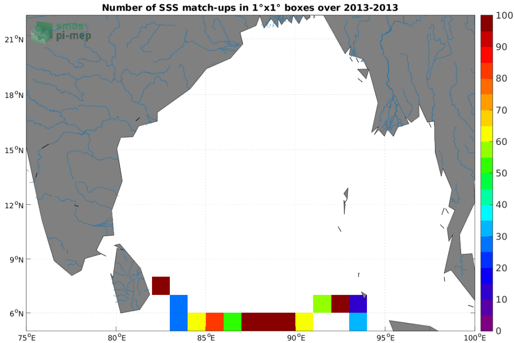
Figure 3: Number of SSS match-ups between Surface drifters SSS and the Aquarius SSS L3 CAP v5 - 7-Day running (JPL) SSS product for the Ganga and Brahmaputra river plumes Pi-MEP region over 1°x1° boxes and for the full satellite product period.
