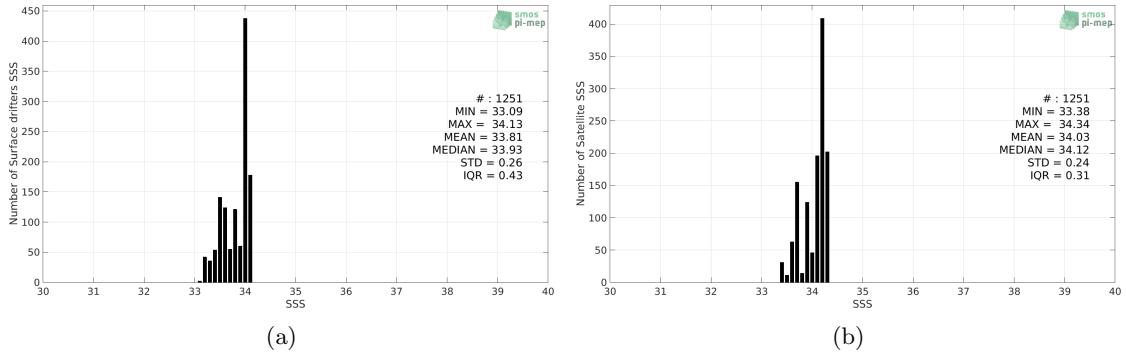
Figure 2: Histograms of SSS from Surface drifters (a) and Aquarius SSS L3 CAP v5 - 7-Day running (JPL) (b) considering all match-up pairs per bins of 0.1 over the Ganga and Brahmaputra river plumes Pi-MEP region and for the full satellite product period.
