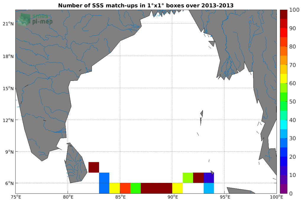
Figure 3: Number of SSS match-ups between Surface drifters SSS and the Aquarius SSS L3 CAP v5 - 7-Day running (JPL) SSS product for the Ganga and Brahmaputra river plumes Pi-MEP region over 1^\circ \times 1^\circ boxes and for the full satellite product period.
