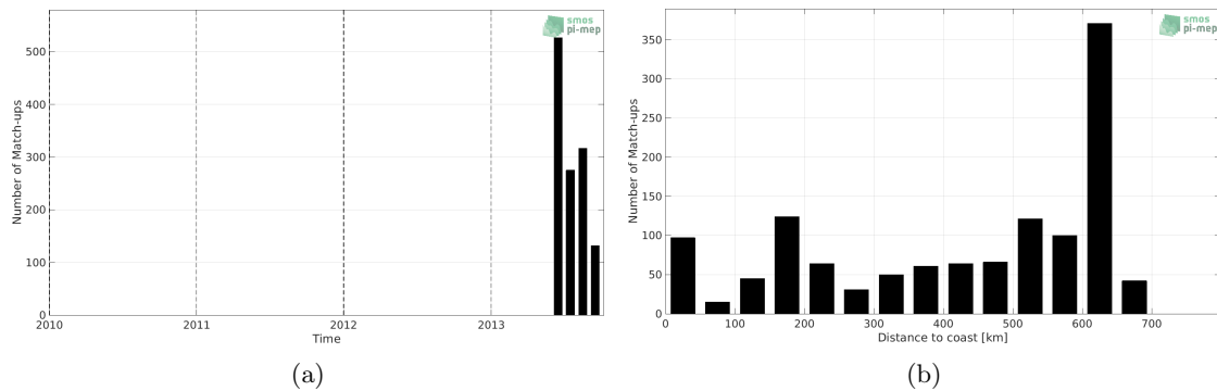
Figure 1: Number of match-ups between Surface drifters and Aquarius SSS L3 CAP v5 - 7-Day running (JPL) SSS as a function of time (a) and as function of the distance to coast (b) over the Ganga and Brahmaputra river plumes Pi-MEP region and for the full satellite product period.
