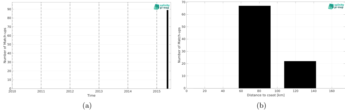
Figure 1: Number of match-ups between TSG (SAMOS) and Aquarius SSS L3 CAP v5 - Monthly (JPL) SSS as a function of time (a) and as function of the distance to coast (b) over the Ganga and Brahmaputra river plumes Pi-MEP region and for the full satellite product period.
