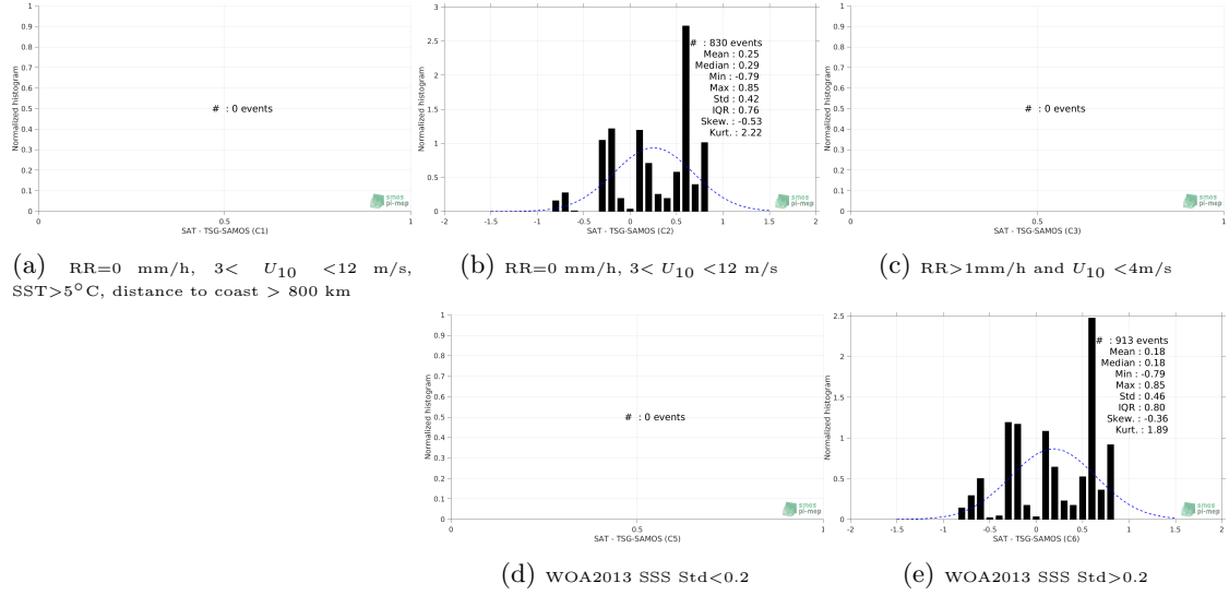
Figure 13: Normalized histogram of \Delta\text{SSS} (Aquarius-L3-JPL-V5-MONTHLY - TSG-SAMOS) for 5 different subdatasets corresponding to: RR=0 mm/h, 3 < U_{10} < 12 m/s, SST > 5^\circ\text{C} , distance to coast > 800 km (a), RR=0 mm/h, 3 < U_{10} < 12 m/s (b), RR > 1\text{mm/h} and U_{10} < 4\text{m/s} (c), WOA2013 SSS Std < 0.2 (d), WOA2013 SSS Std > 0.2 (e).
