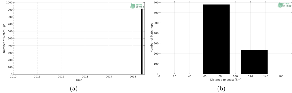
Figure 1: Number of match-ups between TSG-SAMOS and Aquarius-L3-JPL-V5-MONTHLY SSS as a function of time (a) and as function of the distance to coast (b) over the Ganga and Brahmaputra river plumes Pi-MEP region and for the full satellite product period.
