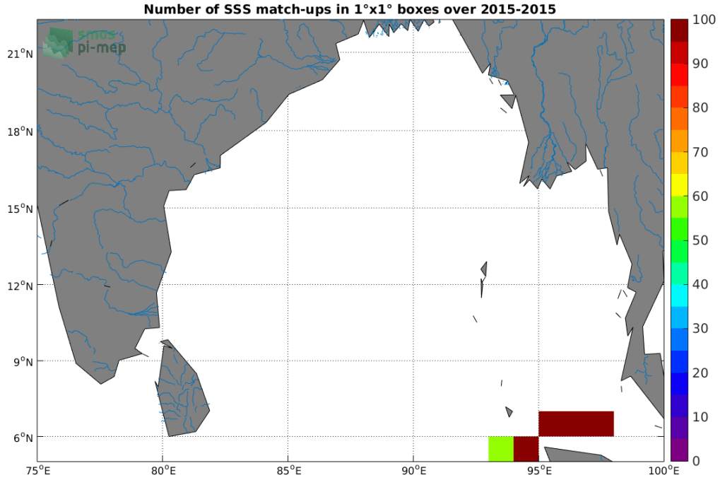
Figure 4: Number of SSS match-ups between TSG-SAMOS SSS and the Aquarius-L3-JPL-V5-MONTHLY SSS product for the Ganga and Brahmaputra river plumes Pi-MEP region over 1^\circ \times 1^\circ boxes and for the full satellite product period.
