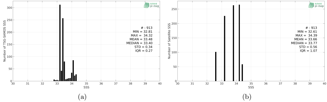
Figure 2: Histograms of SSS from TSG-SAMOS (a) and Aquarius-L3-JPL-V5-MONTHLY (b) considering all match-up pairs per bins of 0.1 over the Ganga and Brahmaputra river plumes Pi-MEP region and for the full satellite product period.
