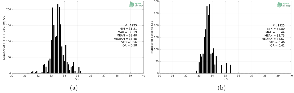
Figure 2: Histograms of SSS from TSG (LEGOS-DM) (a) and Aquarius SSS L3 CAP v5 - Monthly (JPL) (b) considering all match-up pairs per bins of 0.1 over the Ganga and Brahmaputra river plumes Pi-MEP region and for the full satellite product period.
