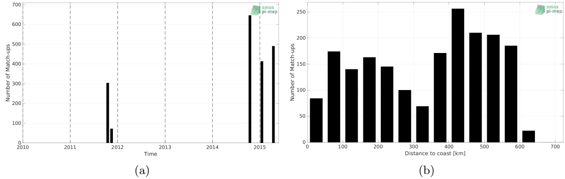
Figure 1: Number of match-ups between TSG (LEGOS-DM) and Aquarius SSS L3 CAP v5 - Monthly (JPL) SSS as a function of time (a) and as function of the distance to coast (b) over the Ganga and Brahmaputra river plumes Pi-MEP region and for the full satellite product period.
