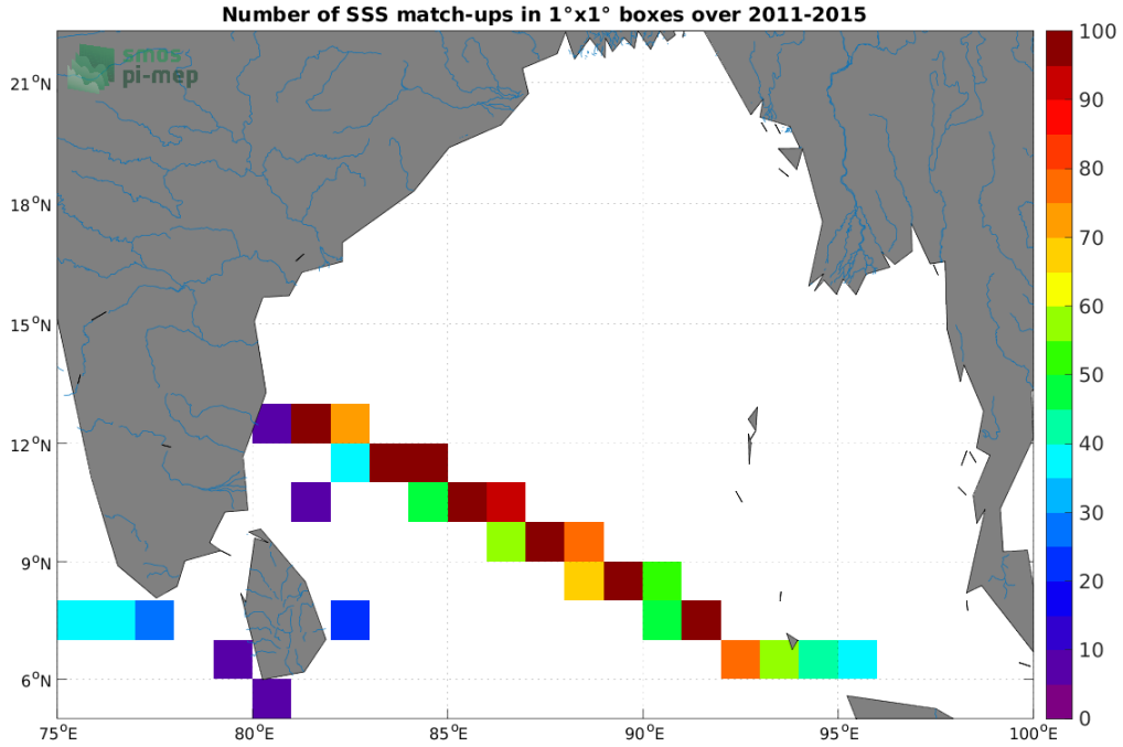
Figure 4: Number of SSS match-ups between TSG (LEGOS-DM) SSS and the Aquarius SSS L3 CAP v5 - Monthly (JPL) SSS product for the Ganga and Brahmaputra river plumes Pi-MEP region over 1°x1° boxes and for the full satellite product period.
