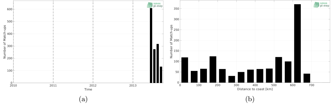
Figure 1: Number of match-ups between Surface drifters and Aquarius SSS L3 CAP v5 - Monthly (JPL) SSS as a function of time (a) and as function of the distance to coast (b) over the Ganga and Brahmaputra river plumes Pi-MEP region and for the full satellite product period.
