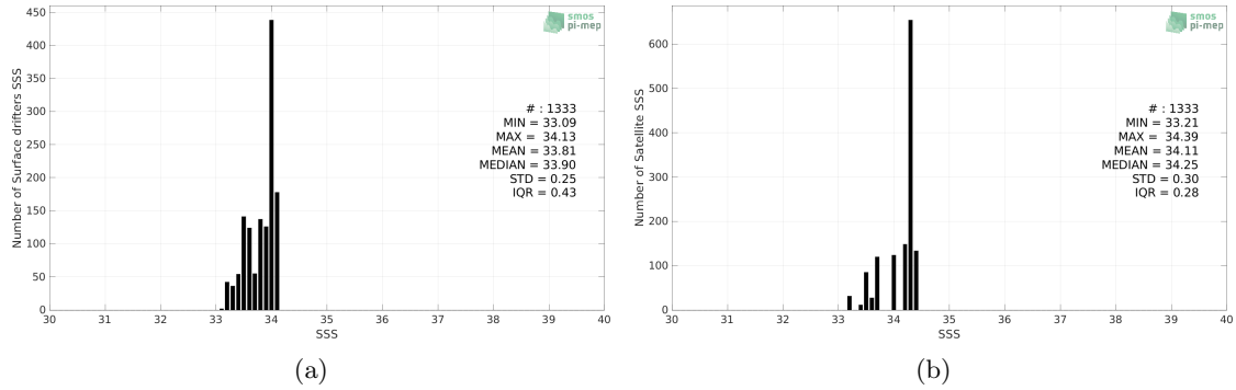
Figure 2: Histograms of SSS from Surface drifters (a) and Aquarius SSS L3 CAP v5 - Monthly (JPL) (b) considering all match-up pairs per bins of 0.1 over the Ganga and Brahmaputra river plumes Pi-MEP region and for the full satellite product period.
