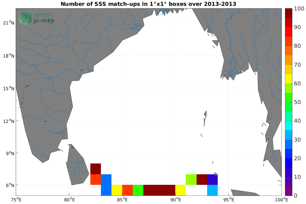
Figure 3: Number of SSS match-ups between Surface drifters SSS and the Aquarius SSS L3 CAP v5 - Monthly (JPL) SSS product for the Ganga and Brahmaputra river plumes Pi-MEP region over 1°x1° boxes and for the full satellite product period.
