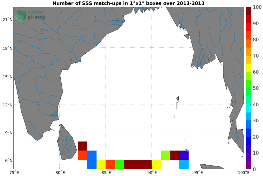
Figure 3: Number of SSS match-ups between Surface drifters SSS and the Aquarius SSS L3 CAP v5 - Monthly (JPL) SSS product for the Ganga and Brahmaputra river plumes Pi-MEP region over 1^\circ \times 1^\circ boxes and for the full satellite product period.
