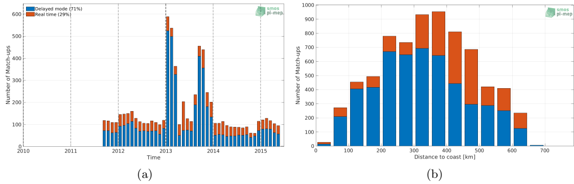
Figure 1: Number of match-ups between Argo and Aquarius SSS L3 CAP v5 - Monthly (JPL) SSS as a function of time (a) and as function of the distance to coast (b) over the Ganga and Brahmaputra river plumes Pi-MEP region and for the full satellite product period.
