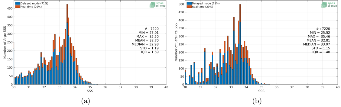
Figure 2: Histograms of SSS from Argo (a) and Aquarius SSS L3 CAP v5 - Monthly (JPL) (b) considering all match-up pairs per bins of 0.1 over the Ganga and Brahmaputra river plumes Pi-MEP region and for the full satellite product period.
