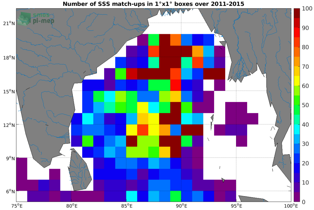
Figure 4: Number of SSS match-ups between Argo SSS and the Aquarius SSS L3 CAP v5 - Monthly (JPL) SSS product for the Ganga and Brahmaputra river plumes Pi-MEP region over 1^\circ \times 1^\circ boxes and for the full satellite product period.
