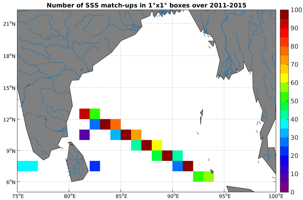
Figure 4: Number of SSS match-ups between TSG-LEGOS-DM SSS and the Aquarius-L3-JPL-V4-7DAY-RUNNING SSS product for the Ganga and Brahmaputra river plumes Pi-MEP region over 1^\circ \times 1^\circ boxes and for the full satellite product period.
