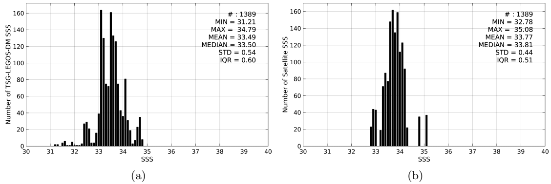
Figure 2: Histograms of SSS from TSG-LEGOS-DM (a) and Aquarius-L3-JPL-V4-7DAY-RUNNING (b) considering all match-up pairs per bins of 0.1 over the Ganga and Brahmaputra river plumes Pi-MEP region and for the full satellite product period.
