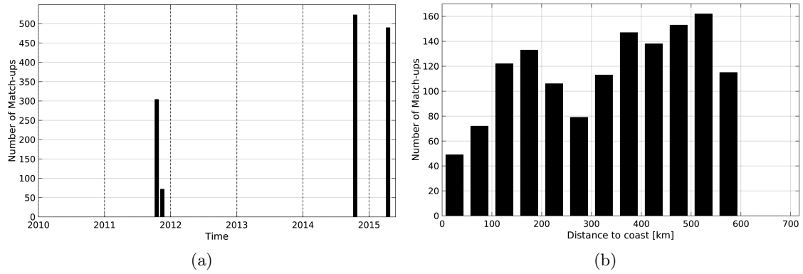
Figure 1: Number of match-ups between TSG-LEGOS-DM and Aquarius-L3-JPL-V4-7DAY-RUNNING SSS as a function of time (a) and as function of the distance to coast (b) over the Ganga and Brahmaputra river plumes Pi-MEP region and for the full satellite product period.
