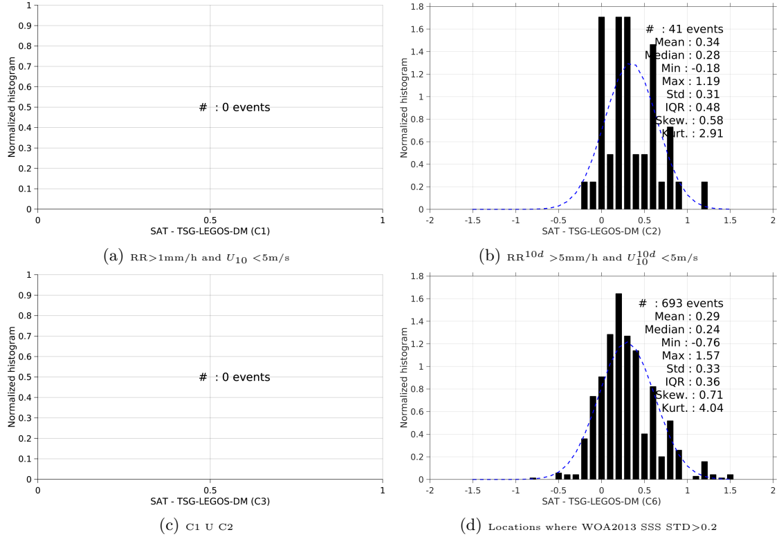
Figure 13: Normalized histogram of \Delta SSS (Aquarius-L3-JPL-V4-7DAY-RUNNING - TSG-LEGOS-DM) for 6 different subdatasets corresponding to: RR > 1mm/h and U_{10} < 5m/s (a), RR^{10d} > 5mm/h and U_{10}^{10d} < 5m/s (b), C1 \cup C2 (c), Locations where WOA2013 SSS STD > 0.2 (d).
