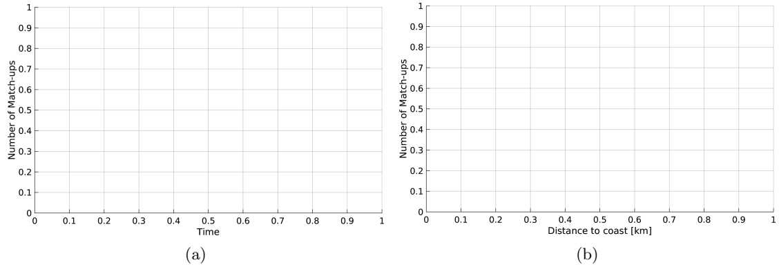
Figure 1: Number of match-ups between TSG-GOSUD-Sailing-ship and Aquarius-L3-JPL-V4-7DAY-RUNNING SSS as a function of time (a) and as function of the distance to coast (b) over the Ganga and Brahmaputra river plumes Pi-MEP region and for the full satellite product period.
