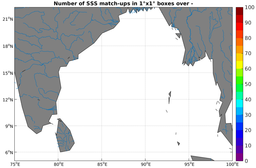
Figure 4: Number of SSS match-ups between TSG-GOSUD-Research-vessel SSS and the Aquarius-L3-JPL-V4-7DAY-RUNNING SSS product for the Ganga and Brahmaputra river plumes Pi-MEP region over 1^\circ \times 1^\circ boxes and for the full satellite product period.
