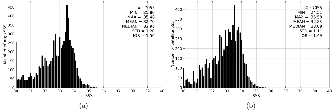
Figure 2: Histograms of SSS from Argo (a) and Aquarius-L3-JPL-V4-7DAY-RUNNING (b) considering all match-up pairs per bins of 0.1 over the Ganga and Brahmaputra river plumes Pi-MEP region and for the full satellite product period.
