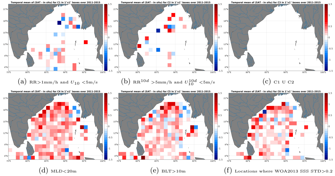
Figure 12: Temporal mean gridded over spatial boxes of size 1^\circ \times 1^\circ of \Delta SSS (Aquarius-L3-JPL-V4-7DAY-RUNNING - Argo) for 6 different subdatasets corresponding to: RR > 1\text{mm/h} and U_{10} < 5\text{m/s} (a), RR^{10d} > 5\text{mm/h} and U_{10}^{10d} < 5\text{m/s} (b), C1 U C2 (c), MLD < 20\text{m} (d), BLT > 10\text{m} (e), Locations where WOA2013 SSS STD > 0.2 (f).
