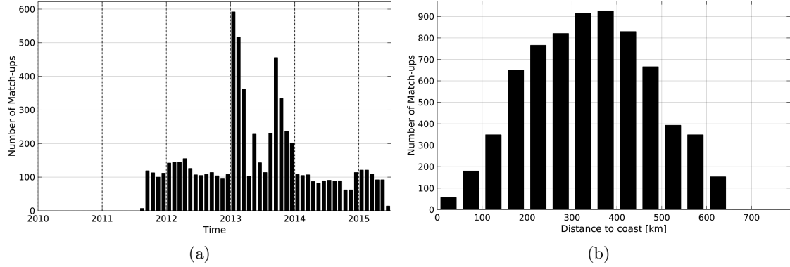
Figure 1: Number of match-ups between Argo and Aquarius-L3-JPL-V4-7DAY-RUNNING SSS as a function of time (a) and as function of the distance to coast (b) over the Ganga and Brahmaputra river plumes Pi-MEP region and for the full satellite product period.
