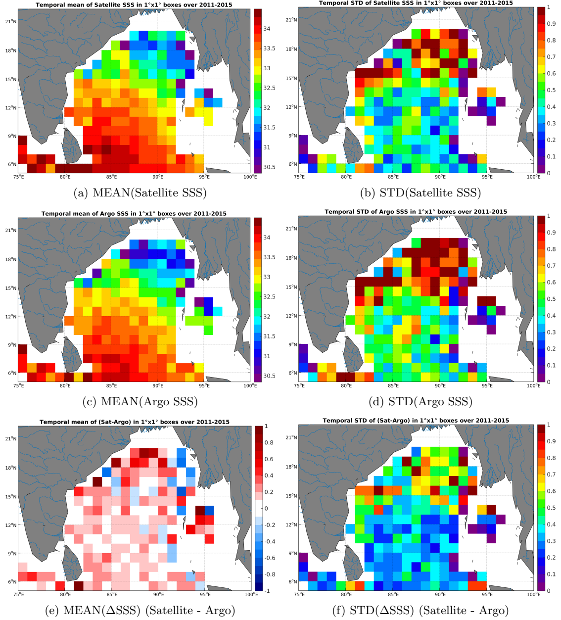
Figure 6: Temporal mean (left) and STD (right) of SSS from Aquarius-L3-JPL-V4-7DAY-RUNNING (top), Argo (middle), and of \Delta SSS (Satellite - Argo). Only match-up pairs are used to generate these maps.
