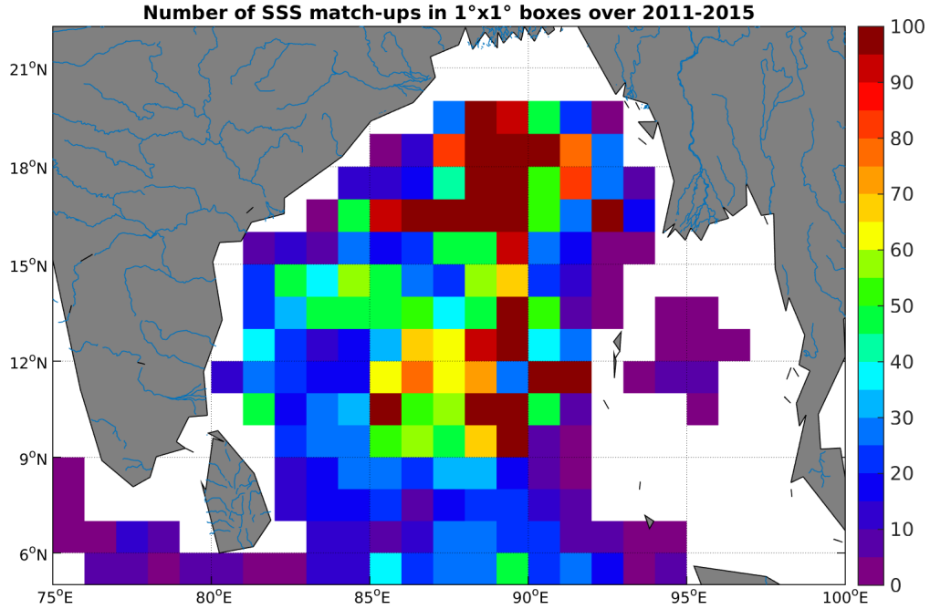
Figure 4: Number of SSS match-ups between Argo SSS and the Aquarius-L3-JPL-V4-7DAY-RUNNING SSS product for the Ganga and Brahmaputra river plumes Pi-MEP region over 1^\circ \times 1^\circ boxes and for the full satellite product period.
