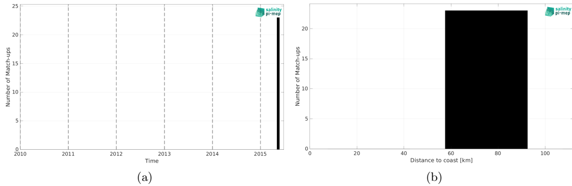
Figure 1: Number of match-ups between TSG (SAMOS) and Aquarius SSS L2 CAP v5 (JPL) SSS as a function of time (a) and as function of the distance to coast (b) over the Ganga and Brahmaputra river plumes Pi-MEP region and for the full satellite product period.
