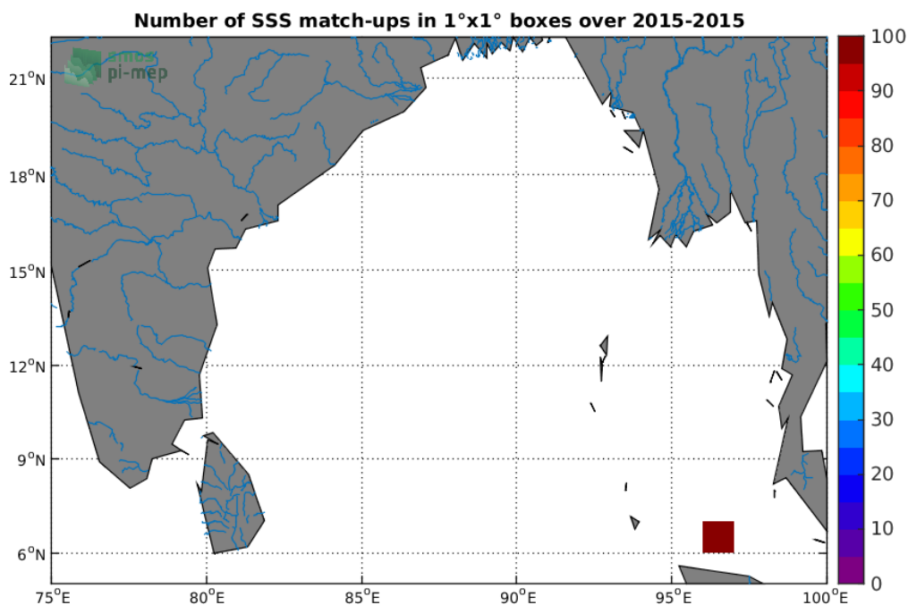
Figure 4: Number of SSS match-ups between TSG-SAMOS SSS and the Aquarius-L2-JPL-V5 SSS product for the Ganga and Brahmaputra river plumes Pi-MEP region over 1^{\circ} \times 1^{\circ} boxes and for the full satellite product period.
