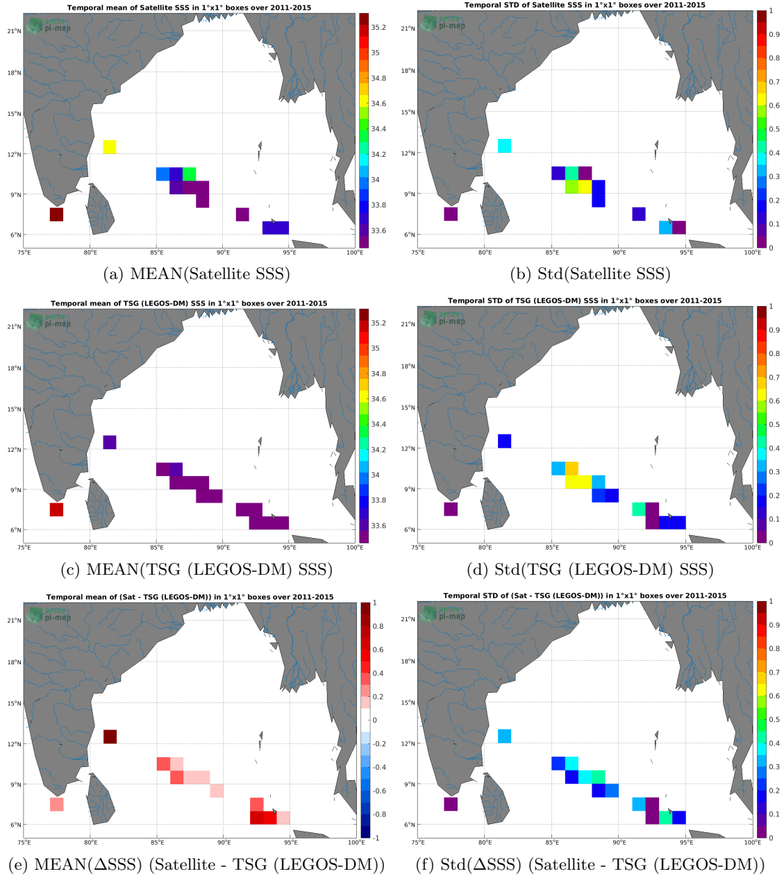
Figure 6: Temporal mean (left) and Std (right) of SSS from Aquarius SSS L2 CAP v5 (JPL) (top), TSG (LEGOS-DM) (middle), and of \Delta SSS (Satellite - TSG (LEGOS-DM)). Only match-pairs are used to generate these maps.
