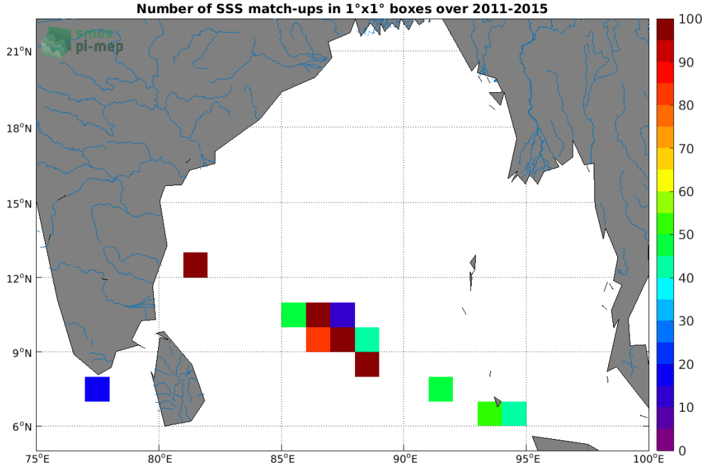
Figure 4: Number of SSS match-ups between TSG (LEGOS-DM) SSS and the Aquarius SSS L2 CAP v5 (JPL) SSS product for the Ganga and Brahmaputra river plumes Pi-MEP region over 1°x1° boxes and for the full satellite product period.
