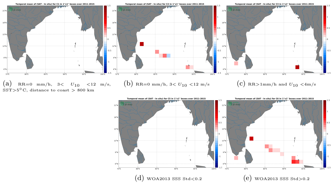
Figure 12: Temporal mean gridded over spatial boxes of size 1°x1° of \Delta SSS (Aquarius SSS L2 CAP v5 (JPL) - TSG (LEGOS-DM)) for 5 different subdatasets corresponding to:RR=0 mm/h, 3 < U_{10} < 12 m/s, SST>5°C, distance to coast > 800 km (a), RR=0 mm/h, 3 < U_{10} < 12 m/s (b), RR>1mm/h and U_{10} < 4 m/s (c), WOA2013 SSS Std<0.2 (d), WOA2013 SSS Std>0.2 (e).
