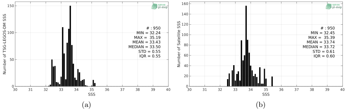
Figure 2: Histograms of SSS from TSG-LEGOS-DM (a) and Aquarius-L2-JPL-V5 (b) considering all match-up pairs per bins of 0.1 over the Ganga and Brahmaputra river plumes Pi-MEP region and for the full satellite product period.
