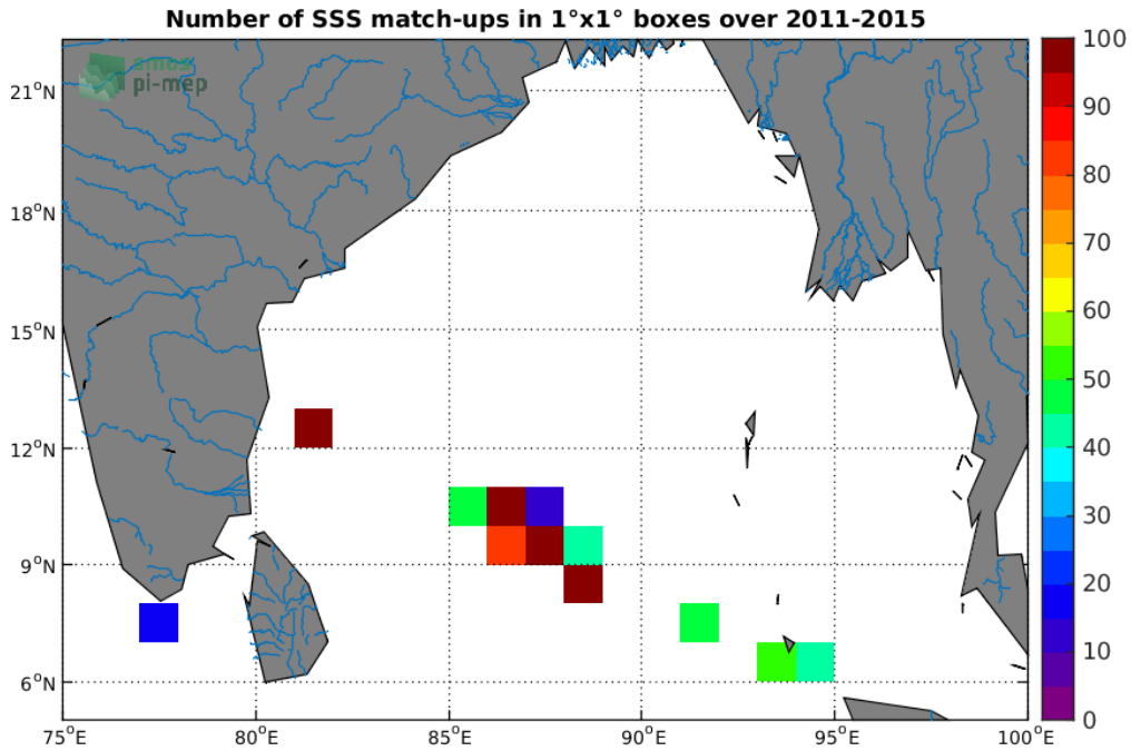
Figure 4: Number of SSS match-ups between TSG-LEGOS-DM SSS and the Aquarius-L2-JPL-V5 SSS product for the Ganga and Brahmaputra river plumes Pi-MEP region over 1°x1° boxes and for the full satellite product period.
