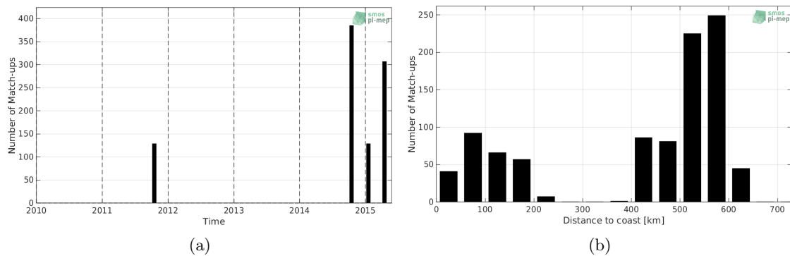
Figure 1: Number of match-ups between TSG-LEGOS-DM and Aquarius-L2-JPL-V5 SSS as a function of time (a) and as function of the distance to coast (b) over the Ganga and Brahmaputra river plumes Pi-MEP region and for the full satellite product period.
