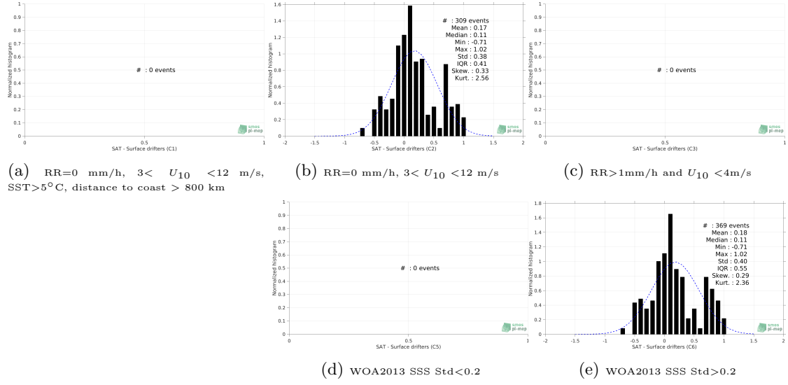
Figure 12: Normalized histogram of \Delta\text{SSS} (Aquarius SSS L2 CAP v5 (JPL) - Surface drifters) for 5 different subdatasets corresponding to: RR=0 mm/h, 3 < U_{10} < 12 m/s, SST > 5^\circ\text{C} , distance to coast > 800 km (a), RR=0 mm/h, 3 < U_{10} < 12 m/s (b), RR > 1 mm/h and U_{10} < 4 m/s (c), WOA2013 SSS Std <0.2 (d), WOA2013 SSS Std >0.2 (e).
