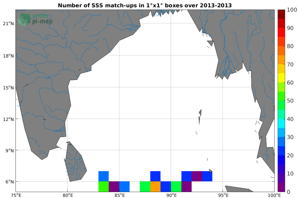
Figure 3: Number of SSS match-ups between Surface drifters SSS and the Aquarius SSS L2 CAP v5 (JPL) SSS product for the Ganga and Brahmaputra river plumes Pi-MEP region over 1^\circ \times 1^\circ boxes and for the full satellite product period.
