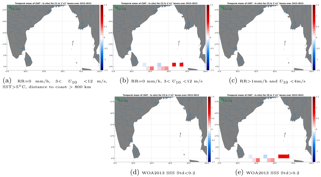
Figure 11: Temporal mean gridded over spatial boxes of size 1°x1° of \Delta SSS (Aquarius SSS L2 CAP v5 (JPL) - Surface drifters) for 5 different subdatasets corresponding to:RR=0 mm/h, 3 < U_{10} < 12 m/s, SST>5°C, distance to coast > 800 km (a), RR=0 mm/h, 3 < U_{10} < 12 m/s (b), RR>1mm/h and U_{10} < 4 m/s (c), WOA2013 SSS Std<0.2 (d), WOA2013 SSS Std>0.2 (e).
