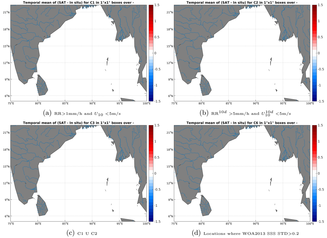
Figure 12: Temporal mean gridded over spatial boxes of size 1^\circ \times 1^\circ of \Delta SSS (AQUARIUS-L2-JPL-V4 - TSG-GOSUD-Sailing-ship) for 4 different subdatasets corresponding to: RR > 1mm/h and U_{10} < 5 m/s (a), RR 10d > 5mm/h and U_{10}^{10d} < 5 m/s (b), C1 U C2 (c), Locations where WOA2013 SSS STD > 0.2 (d).
