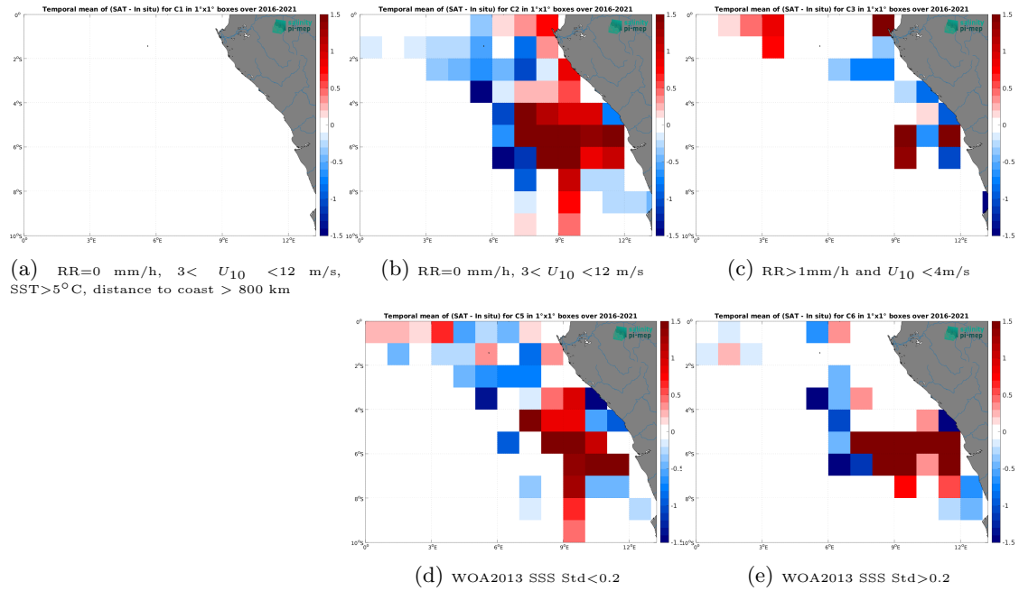
Figure 12: Temporal mean gridded over spatial boxes of size 1^\circ \times 1^\circ of \Delta SSS (SMOS SSS L4 v1 - Weekly (CMEMS-CNR) - TSG (LEGOS-DM)) for 5 different subdatasets corresponding to:RR=0 mm/h, 3 < U_{10} < 12 m/s, SST > 5^\circ\text{C} , distance to coast > 800 km (a), RR=0 mm/h, 3 < U_{10} < 12 m/s (b), RR > 1 mm/h and U_{10} < 4 m/s (c), WOA2013 SSS Std < 0.2 (d), WOA2013 SSS Std > 0.2 (e).
