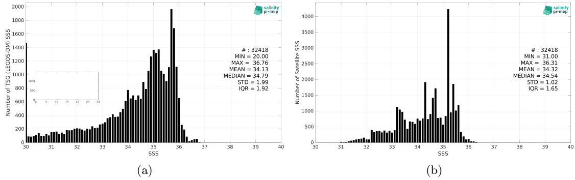
Figure 2: Histograms of SSS from TSG (LEGOS-DM) (a) and SMOS SSS L4 v1 - Weekly (CMEMS-CNR) (b) considering all match-up pairs per bins of 0.1 over the Congo river plume Pi-MEP region and for the full satellite product period.
