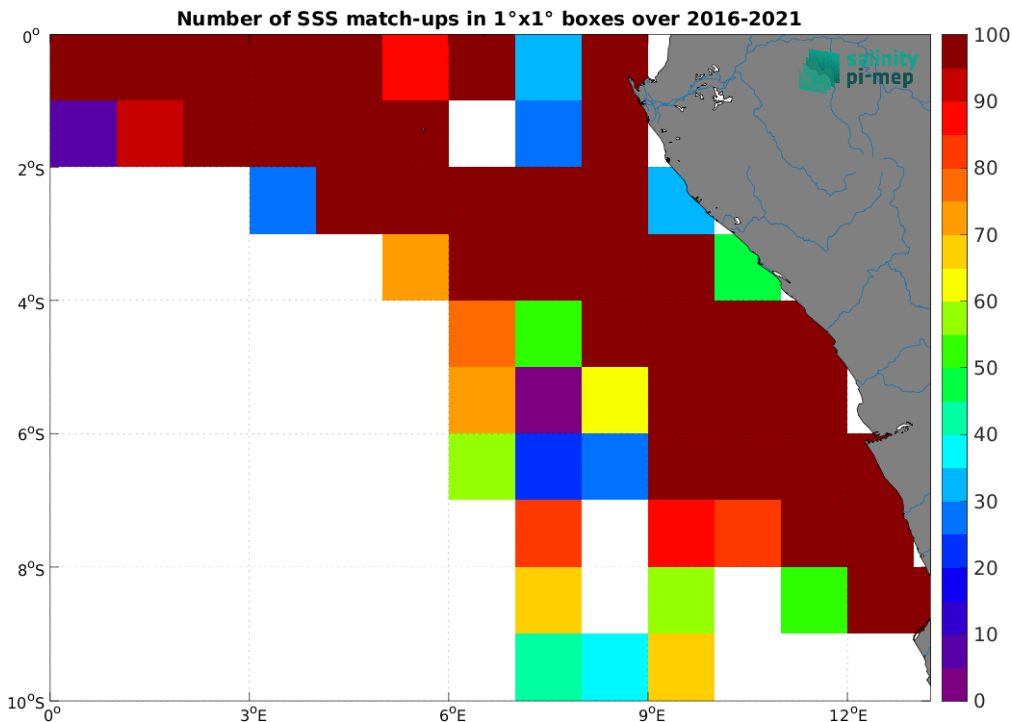
Figure 4: Number of SSS match-ups between TSG (LEGOS-DM) SSS and the SMOS SSS L4 v1 - Weekly (CMEMS-CNR) SSS product for the Congo river plume Pi-MEP region over 1^{\circ} \times 1^{\circ} boxes and for the full satellite product period.
