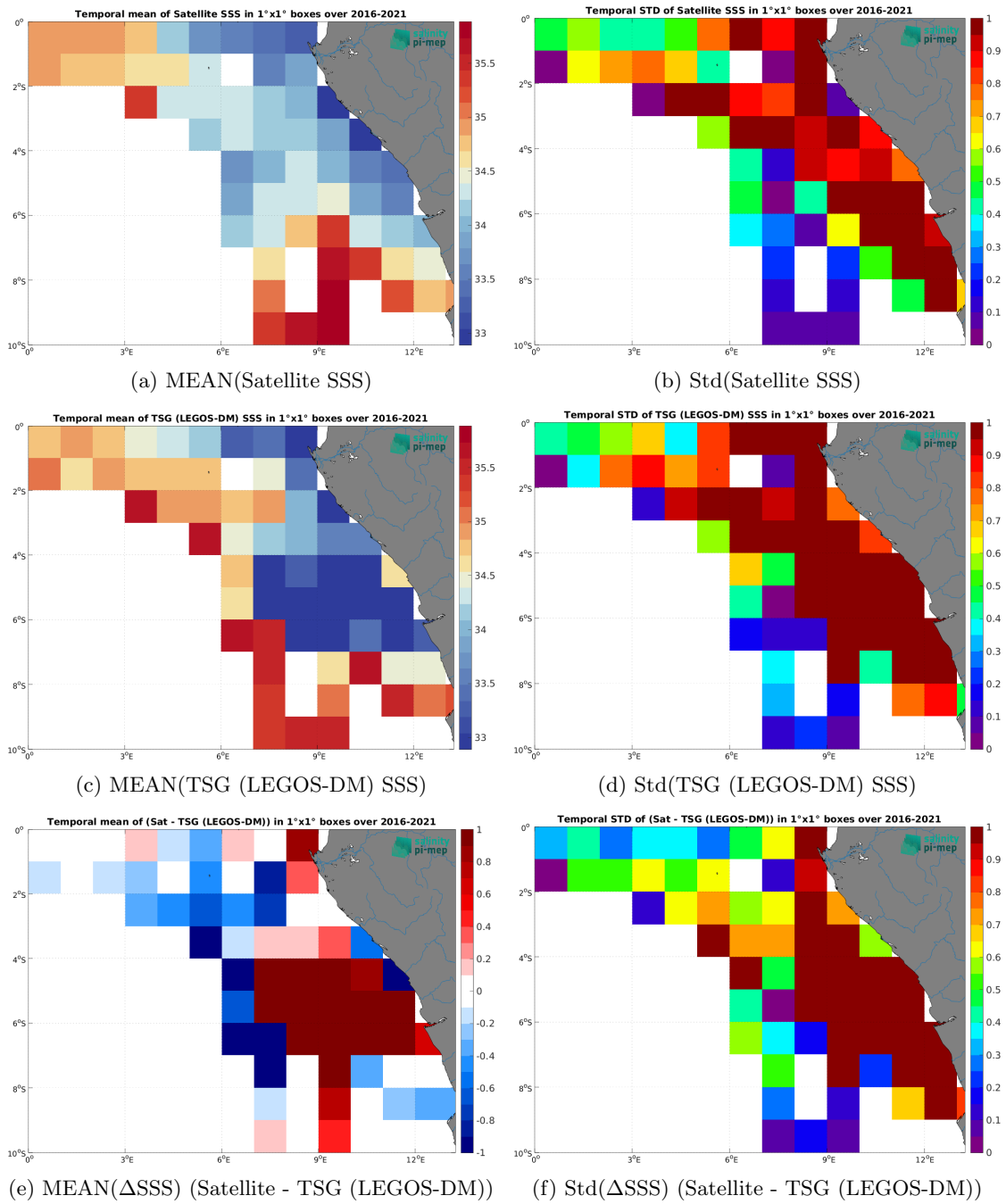
Figure 6: Temporal mean (left) and Std (right) of SSS from SMOS SSS L4 v1 - Weekly (CMEMS-CNR) (top), TSG (LEGOS-DM) (middle), and of \Delta SSS (Satellite - TSG (LEGOS-DM)). Only match-up pairs are used to generate these maps.
