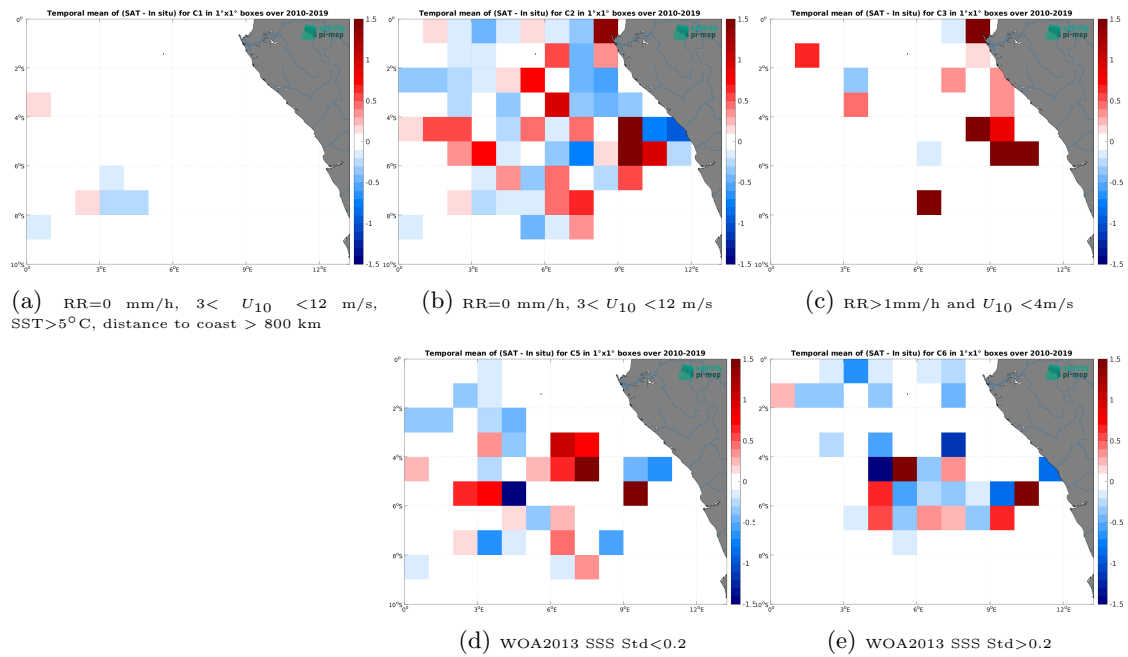
Figure 12: Temporal mean gridded over spatial boxes of size 1^\circ \times 1^\circ of \Delta SSS (SMOS SSS L4 v1 - Weekly (CMEMS-CNR) - TSG (GOSUD-Research-vessel)) for 5 different subdatasets corresponding to:RR=0 mm/h, 3 < U_{10} < 12 m/s, SST > 5°C, distance to coast > 800 km (a), RR=0 mm/h, 3 < U_{10} < 12 m/s (b), RR > 1mm/h and U_{10} < 4 m/s (c), WOA2013 SSS Std < 0.2 (d), WOA2013 SSS Std > 0.2 (e).
