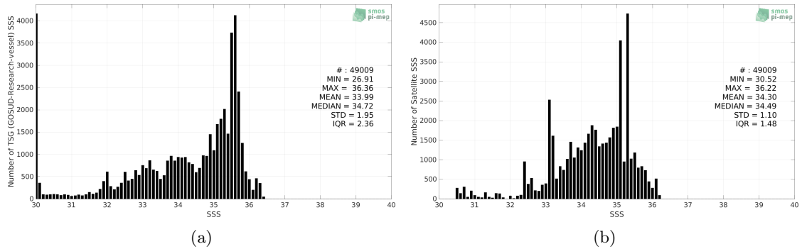
Figure 2: Histograms of SSS from TSG (GOSUD-Research-vessel) (a) and SMOS SSS L4 v1 - Weekly (CMEMS-CNR) (b) considering all match-up pairs per bins of 0.1 over the Congo river plume Pi-MEP region and for the full satellite product period.
