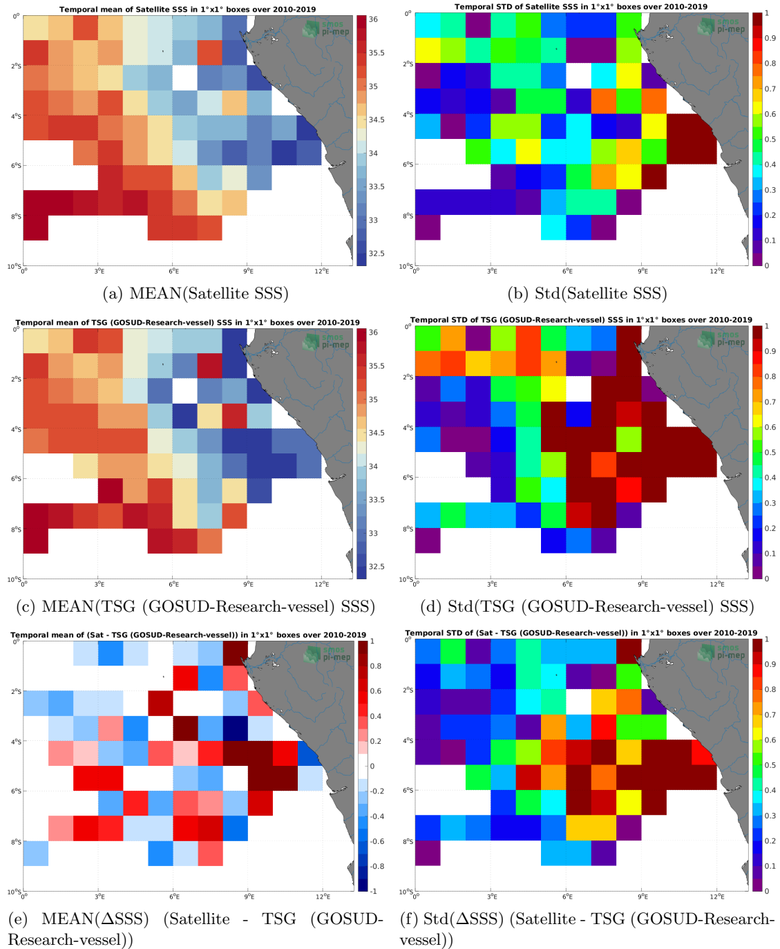
Figure 6: Temporal mean (left) and Std (right) of SSS from SMOS SSS L4 v1 - Weekly (CMEMS-CNR) (top), TSG (GOSUD-Research-vessel) (middle), and of \Delta SSS (Satellite - TSG (GOSUD-Research-vessel)). Only match-up pairs are used to generate these maps.
