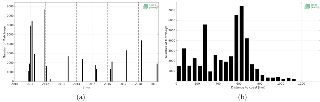
Figure 1: Number of match-ups between TSG (GOSUD-Research-vessel) and SMOS SSS L4 v1 - Weekly (CMEMS-CNR) SSS as a function of time (a) and as function of the distance to coast (b) over the Congo river plume Pi-MEP region and for the full satellite product period.
