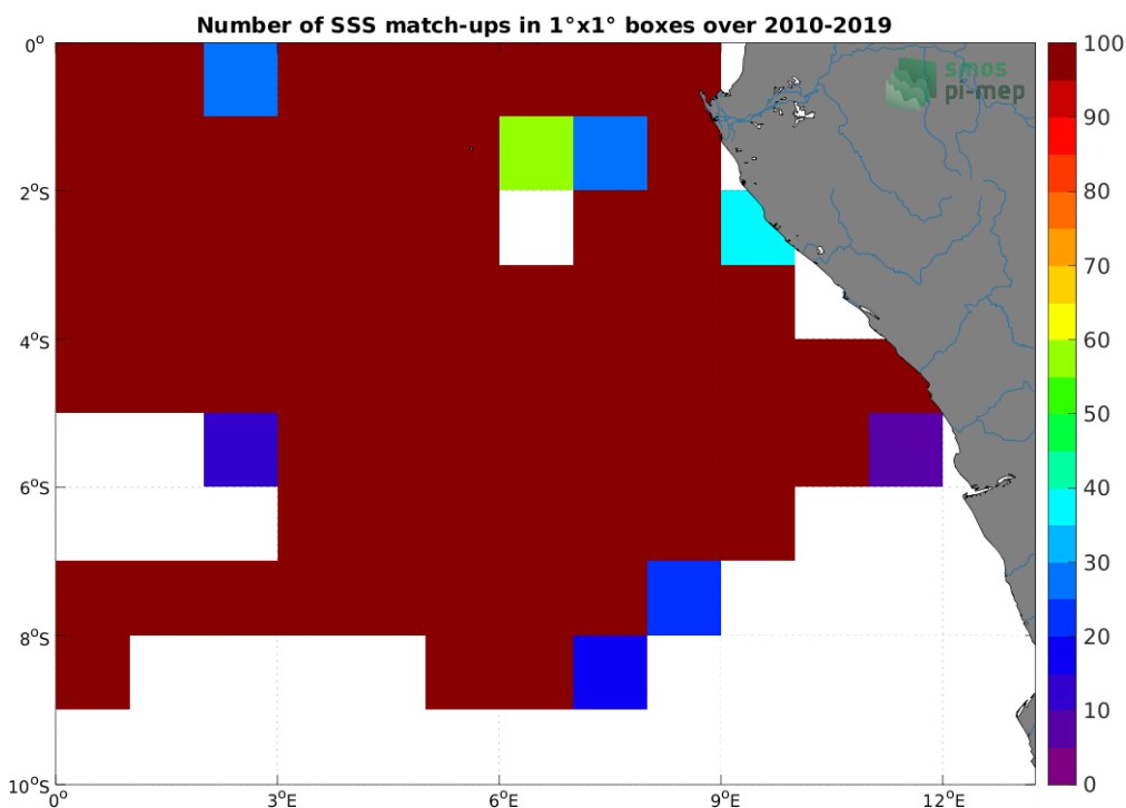
Figure 4: Number of SSS match-ups between TSG (GOSUD-Research-vessel) SSS and the SMOS SSS L4 v1 - Weekly (CMEMS-CNR) SSS product for the Congo river plume Pi-MEP region over 1^{\circ} \times 1^{\circ} boxes and for the full satellite product period.
