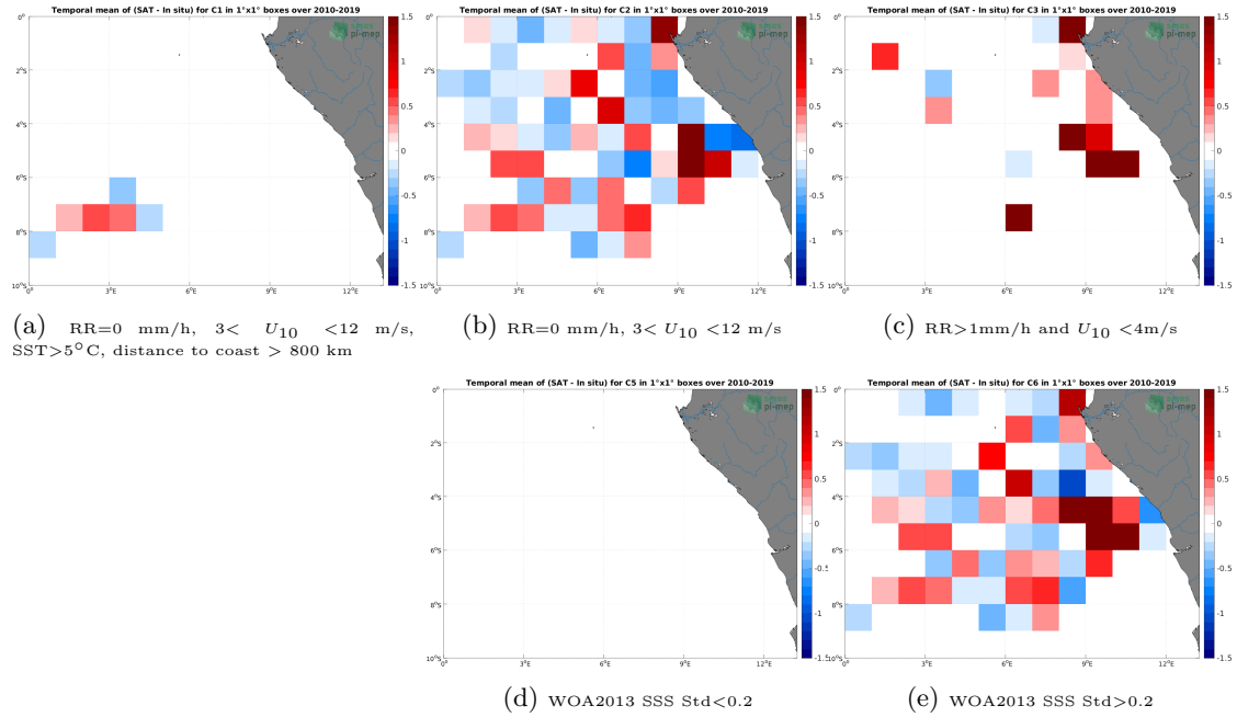
Figure 12: Temporal mean gridded over spatial boxes of size 1^{\circ}\times 1^{\circ} of \Delta SSS (SMOS SSS L4 v1 - Weekly (CMEMS-CNR) - TSG (GOSUD-Research-vessel)) for 5 different subdatasets corresponding to:RR=0 mm/h, 3 < U_{10} < 12 m/s, SST >5^{\circ}\text{C} , distance to coast > 800 km (a), RR=0 mm/h, 3 < U_{10} < 12 m/s (b), RR >1 mm/h and U_{10} < 4 m/s (c), WOA2013 SSS Std <0.2 (d), WOA2013 SSS Std >0.2 (e).
