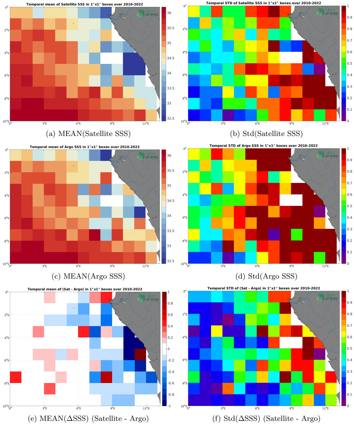
Figure 6: Temporal mean (left) and Std (right) of SSS from SMOS SSS L4 v1 - Weekly (CMEMS-CNR) (top), Argo (middle), and of \Delta SSS (Satellite - Argo). Only match-up pairs are used to generate these maps.
