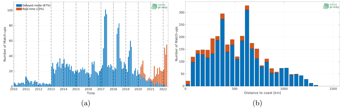
Figure 1: Number of match-ups between Argo and SMOS SSS L4 v1 - Weekly (CMEMS-CNR) SSS as a function of time (a) and as function of the distance to coast (b) over the Congo river plume Pi-MEP region and for the full satellite product period.
