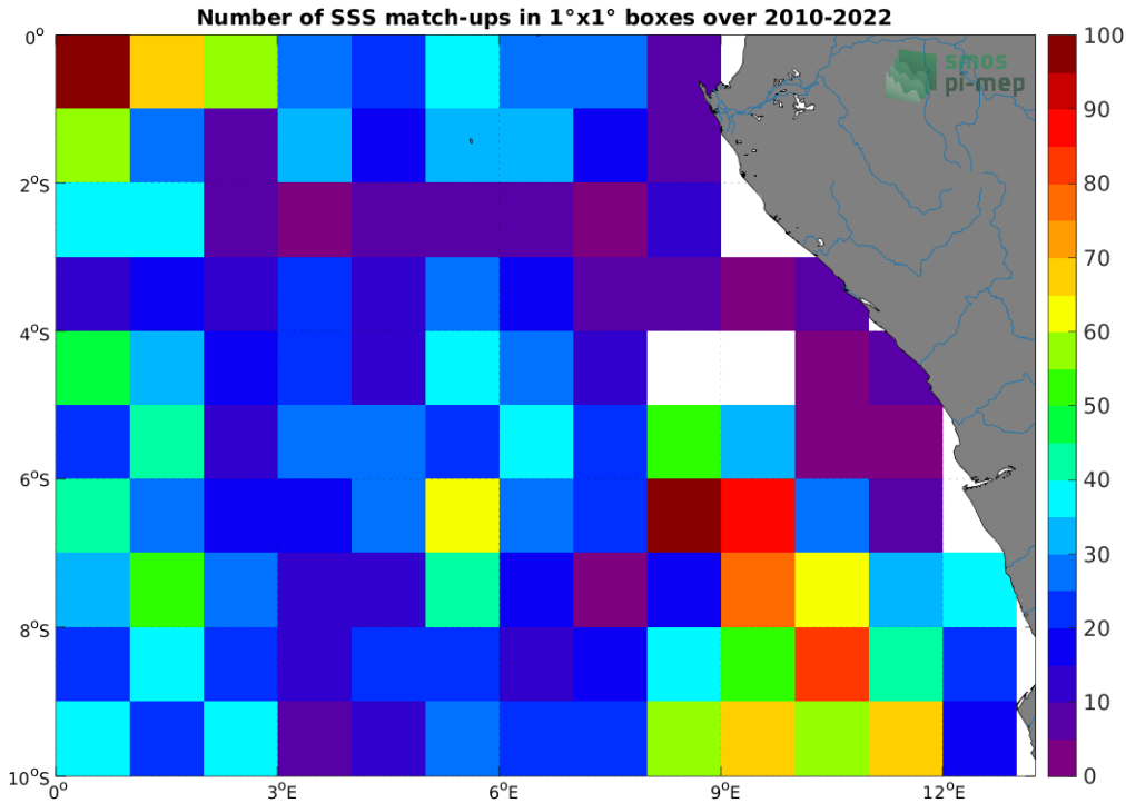
Figure 4: Number of SSS match-ups between Argo SSS and the SMOS SSS L4 v1 - Weekly (CMEMS-CNR) SSS product for the Congo river plume Pi-MEP region over 1^\circ \times 1^\circ boxes and for the full satellite product period.
