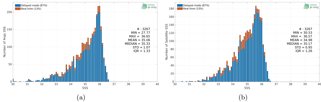
Figure 2: Histograms of SSS from Argo (a) and SMOS SSS L4 v1 - Weekly (CMEMS-CNR) (b) considering all match-up pairs per bins of 0.1 over the Congo river plume Pi-MEP region and for the full satellite product period.
