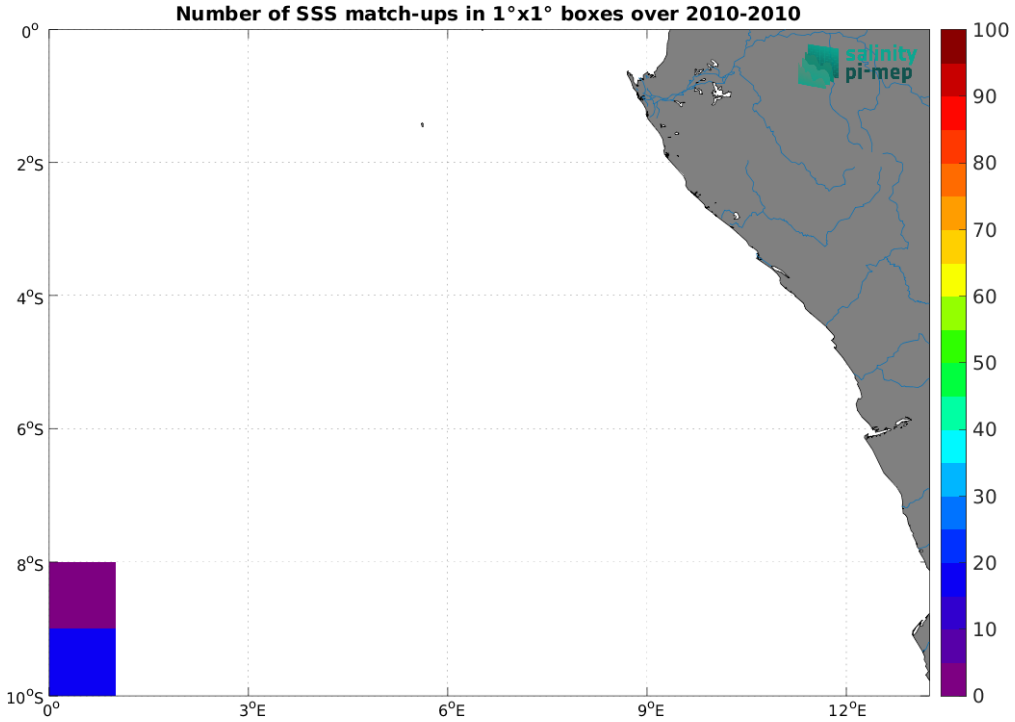
Figure 5: Number of SSS match-ups between TSG (SAMOS) SSS and the SMOS SSS L4 v1 - Monthly (CMEMS-CNR) SSS product for the Congo river plume Pi-MEP region over 1^\circ \times 1^\circ boxes and for the full satellite product period.
