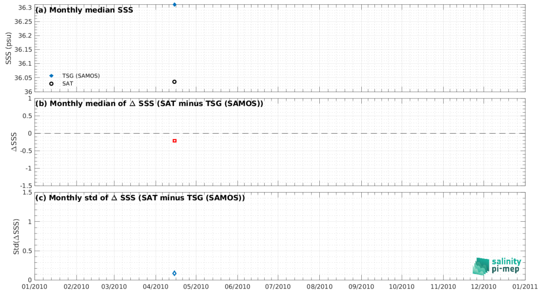
Figure 8: Time series of the monthly median SSS (top), median of \Delta SSS (Satellite - TSG (SAMOS)) and Std of \Delta SSS (Satellite - TSG (SAMOS)) over the Congo river plume Pi-MEP region considering all match-ups collected by the Pi-MEP.
