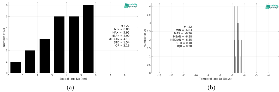
Figure 6: Histograms of the spatial (a) and temporal (b) lags between the location/time of the TSG (SAMOS) measurement and the date of the corresponding SMOS SSS L4 v1 - Monthly (CMEMS-CNR) SSS pixel.
