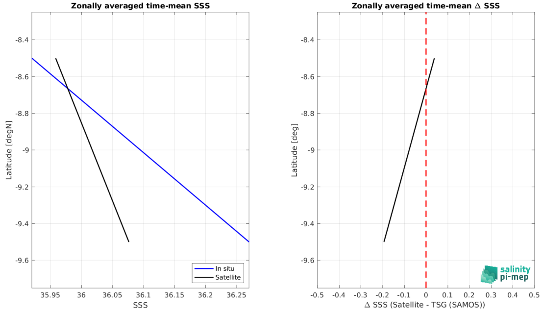
Figure 9: Left panel: Zonal mean SSS from SMOS SSS L4 v1 - Monthly (CMEMS-CNR) satellite product (black) and from TSG (SAMOS) (blue). Right panel: Zonal mean of \Delta SSS (Satellite - TSG (SAMOS)) for all the collected Pi-MEP match-up pairs estimated over the full satellite product period.
