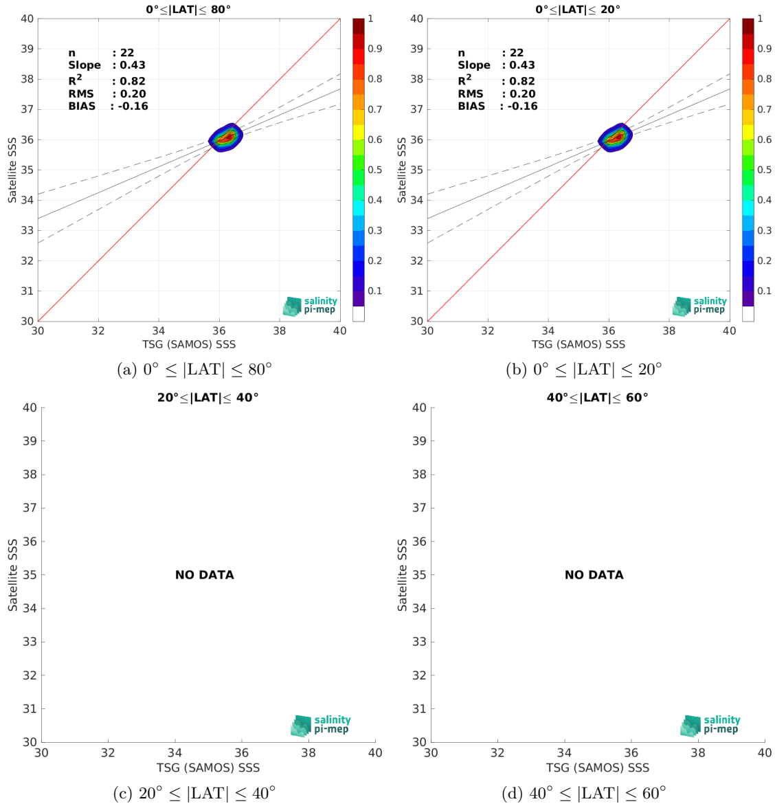
Figure 10: Contour maps of the concentration of SMOS SSS L4 v1 - Monthly (CMEMS-CNR) SSS (y-axis) versus TSG (SAMOS) SSS (x-axis) at match-up pairs for different latitude bands. For each plot, the red line shows x=y . The black thin and dashed lines indicate a linear fit through the data cloud and the \pm 95\% confidence levels, respectively. The number match-up pairs n , the slope and R^2 coefficient of the linear fit, the root mean square (RMS) and the mean bias between satellite and in situ data are indicated for each latitude band in each plots.
