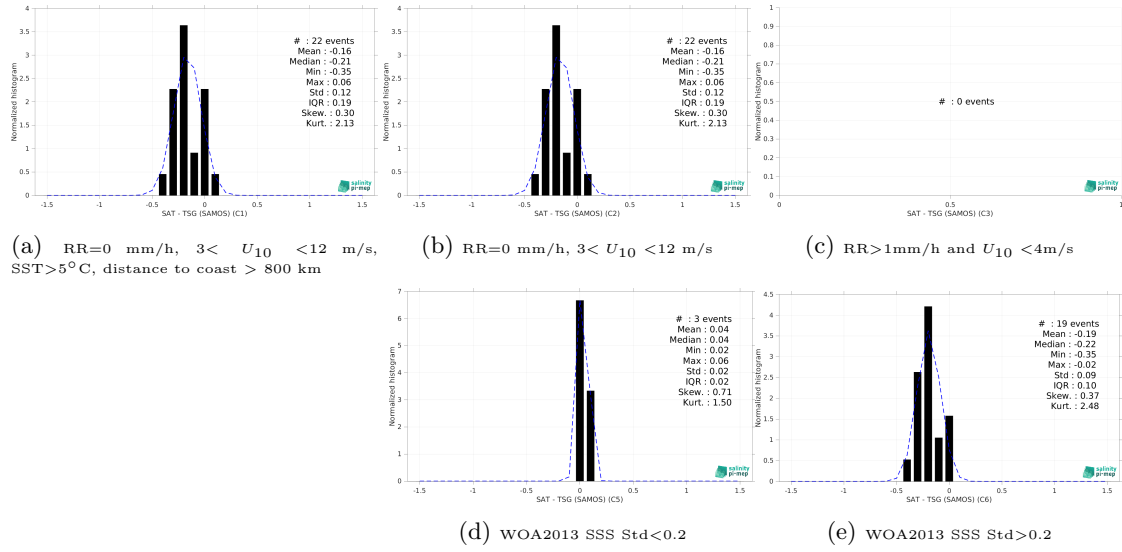
Figure 15: Normalized histogram of \Delta SSS (SMOS SSS L4 v1 - Monthly (CMEMS-CNR) - TSG (SAMOS)) for 5 different subdatasets corresponding to: RR=0 mm/h, 3 < U_{10} < 12 m/s, SST>5°C, distance to coast > 800 km (a), RR=0 mm/h, 3 < U_{10} < 12 m/s (b), RR>1mm/h and U_{10} < 4 m/s (c), WOA2013 SSS Std<0.2 (d), WOA2013 SSS Std>0.2 (e).
