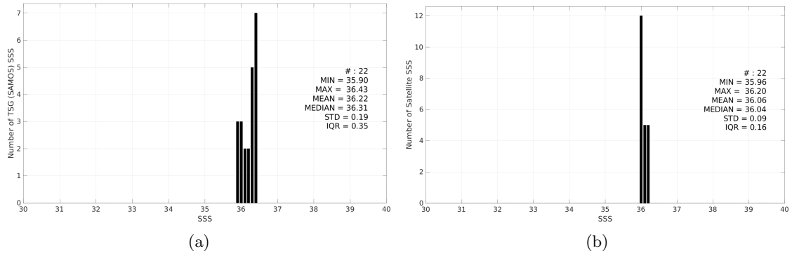
Figure 3: Histograms of SSS from TSG (SAMOS) (a) and SMOS SSS L4 v1 - Monthly (CMEMS-CNR) (b) considering all match-up pairs per bins of 0.1 over the Congo river plume Pi-MEP region and for the full satellite product period.
