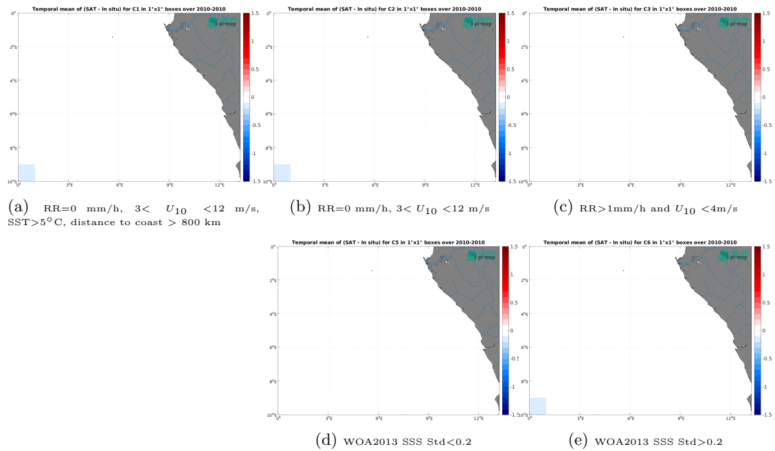
Figure 14: Temporal mean gridded over spatial boxes of size 1^\circ \times 1^\circ of \Delta SSS (SMOS SSS L4 v1 - Monthly (CMEMS-CNR) - TSG (SAMOS)) for 5 different subdatasets corresponding to:RR=0 mm/h, 3 < U_{10} < 12 m/s, SST >5^\circ\text{C} , distance to coast > 800 km (a), RR=0 mm/h, 3 < U_{10} < 12 m/s (b), RR >1 mm/h and U_{10} < 4 m/s (c), WOA2013 SSS Std <0.2 (d), WOA2013 SSS Std >0.2 (e).
