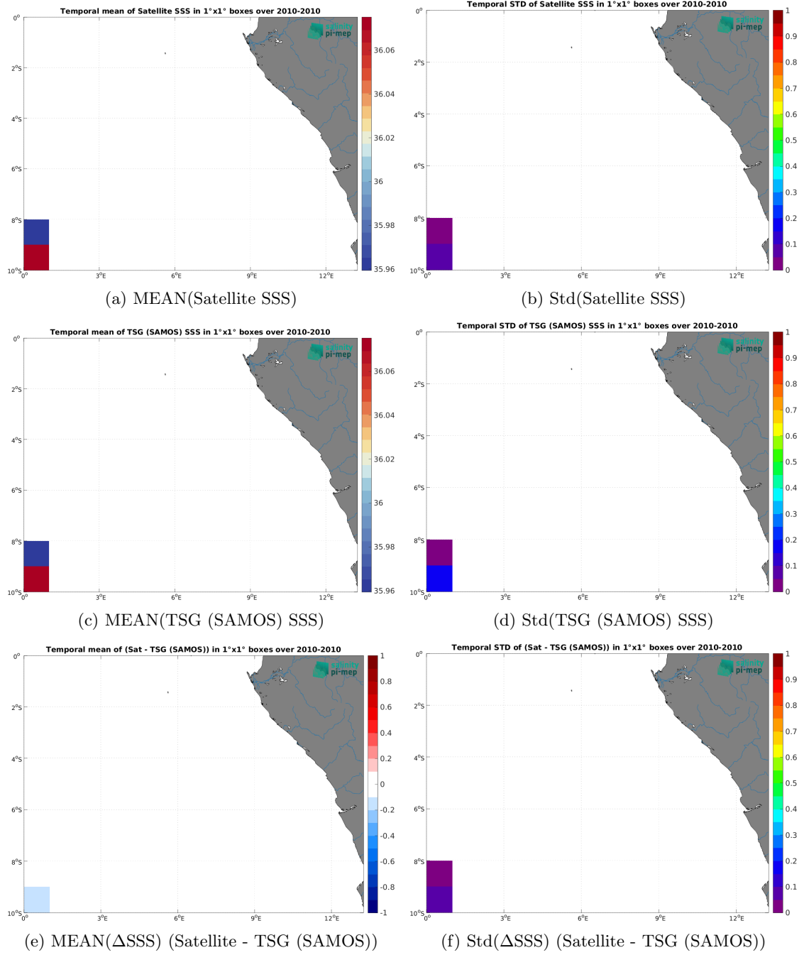
Figure 7: Temporal mean (left) and Std (right) of SSS from SMOS SSS L4 v1 - Monthly (CMEMS-CNR) (top), TSG (SAMOS) (middle), and of \Delta SSS (Satellite - TSG (SAMOS)). Only match-up pairs are used to generate these maps.
