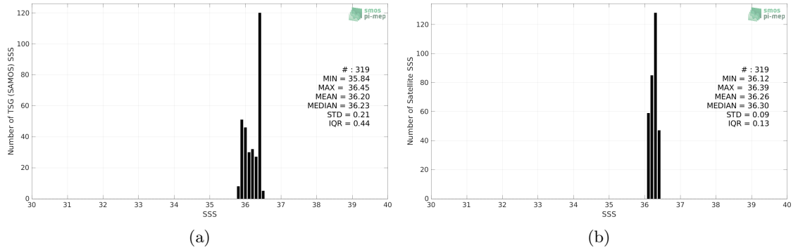
Figure 2: Histograms of SSS from TSG (SAMOS) (a) and SMOS SSS L4 v1 - Monthly (CMEMS-CNR) (b) considering all match-up pairs per bins of 0.1 over the Congo river plume Pi-MEP region and for the full satellite product period.
