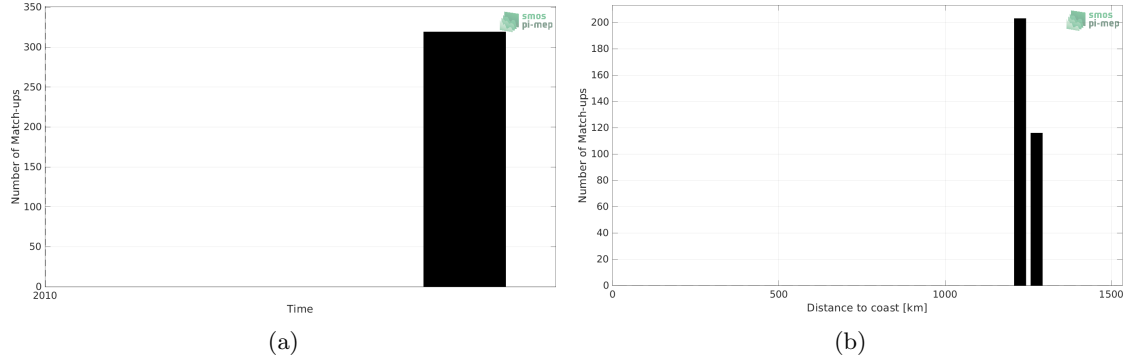
Figure 1: Number of match-ups between TSG (SAMOS) and SMOS SSS L4 v1 - Monthly (CMEMS-CNR) SSS as a function of time (a) and as function of the distance to coast (b) over the Congo river plume Pi-MEP region and for the full satellite product period.
