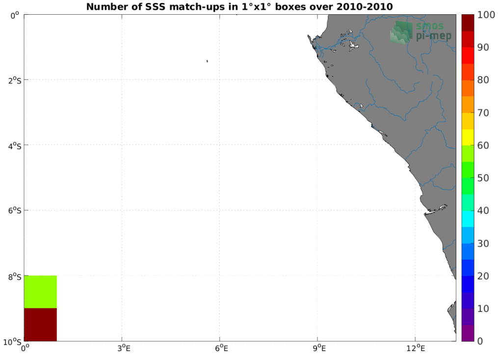
Figure 4: Number of SSS match-ups between TSG (SAMOS) SSS and the SMOS SSS L4 v1 - Monthly (CMEMS-CNR) SSS product for the Congo river plume Pi-MEP region over 1^\circ \times 1^\circ boxes and for the full satellite product period.
