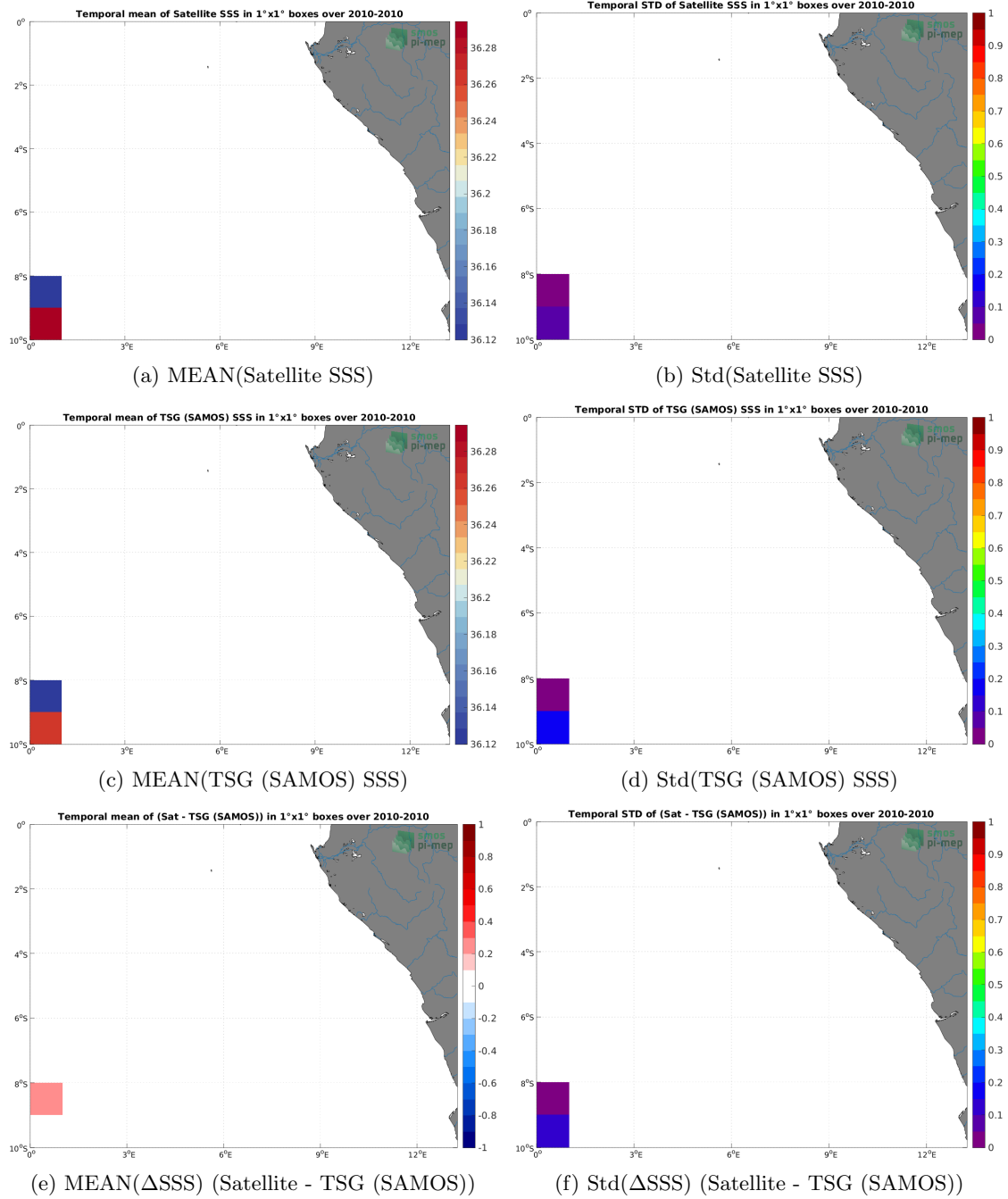
Figure 6: Temporal mean (left) and Std (right) of SSS from SMOS SSS L4 v1 - Monthly (CMEMS-CNR) (top), TSG (SAMOS) (middle), and of \Delta SSS (Satellite - TSG (SAMOS)). Only match-up pairs are used to generate these maps.
