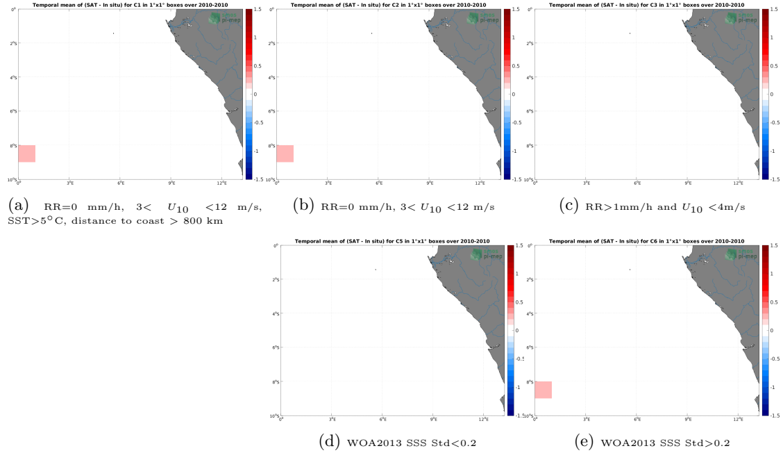
Figure 12: Temporal mean gridded over spatial boxes of size 1^\circ \times 1^\circ of \Delta SSS (SMOS SSS L4 v1 - Monthly (CMEMS-CNR) - TSG (SAMOS)) for 5 different subdatasets corresponding to:RR=0 mm/h, 3 < U_{10} < 12 m/s, SST >5^\circ C, distance to coast > 800 km (a), RR=0 mm/h, 3 < U_{10} < 12 m/s (b), RR >1 mm/h and U_{10} < 4 m/s (c), WOA2013 SSS Std <0.2 (d), WOA2013 SSS Std >0.2 (e).
