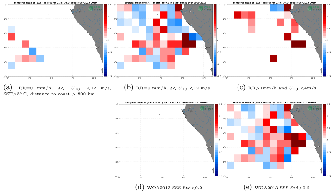
Figure 12: Temporal mean gridded over spatial boxes of size 1^\circ \times 1^\circ of \Delta SSS (SMOS SSS L4 v1 - Monthly (CMEMS-CNR) - TSG (GOSUD-Research-vessel)) for 5 different subdatasets corresponding to: RR=0 mm/h, 3 < U_{10} < 12 m/s, SST > 5^\circ\text{C} , distance to coast > 800 km (a), RR=0 mm/h, 3 < U_{10} < 12 m/s (b), RR > 1 mm/h and U_{10} < 4 m/s (c), WOA2013 SSS Std < 0.2 (d), WOA2013 SSS Std > 0.2 (e).
