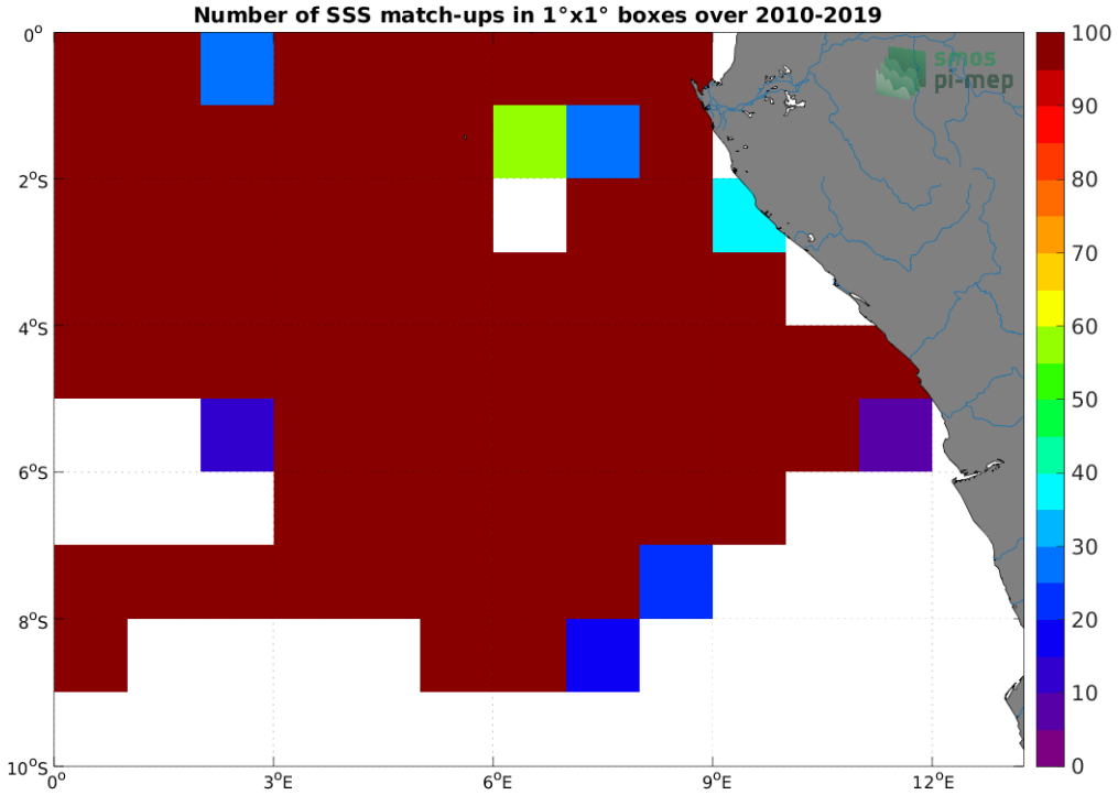
Figure 4: Number of SSS match-ups between TSG (GOSUD-Research-vessel) SSS and the SMOS SSS L4 v1 - Monthly (CMEMS-CNR) SSS product for the Congo river plume Pi-MEP region over 1^\circ \times 1^\circ boxes and for the full satellite product period.
