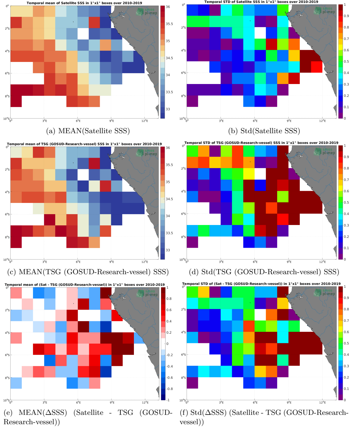
Figure 6: Temporal mean (left) and Std (right) of SSS from SMOS SSS L4 v1 - Monthly (CMEMS-CNR) (top), TSG (GOSUD-Research-vessel) (middle), and of \Delta SSS (Satellite - TSG (GOSUD-Research-vessel)). Only match-up pairs are used to generate these maps.
