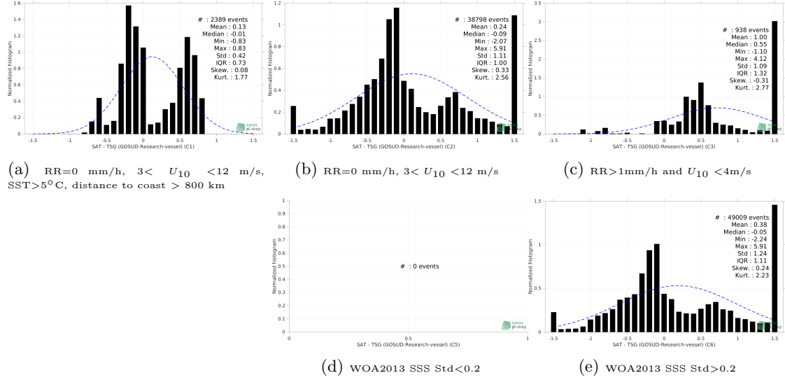
Figure 13: Normalized histogram of \Delta\text{SSS} (SMOS SSS L4 v1 - Monthly (CMEMS-CNR) - TSG (GOSUD-Research-vessel)) for 5 different subdatasets corresponding to: RR=0 mm/h, 3 < U_{10} < 12 m/s, SST > 5^\circ\text{C} , distance to coast > 800 km (a), RR=0 mm/h, 3 < U_{10} < 12 m/s (b), RR > 1\text{mm/h} and U_{10} < 4\text{m/s} (c), WOA2013 SSS \text{Std} < 0.2 (d), WOA2013 SSS \text{Std} > 0.2 (e).
