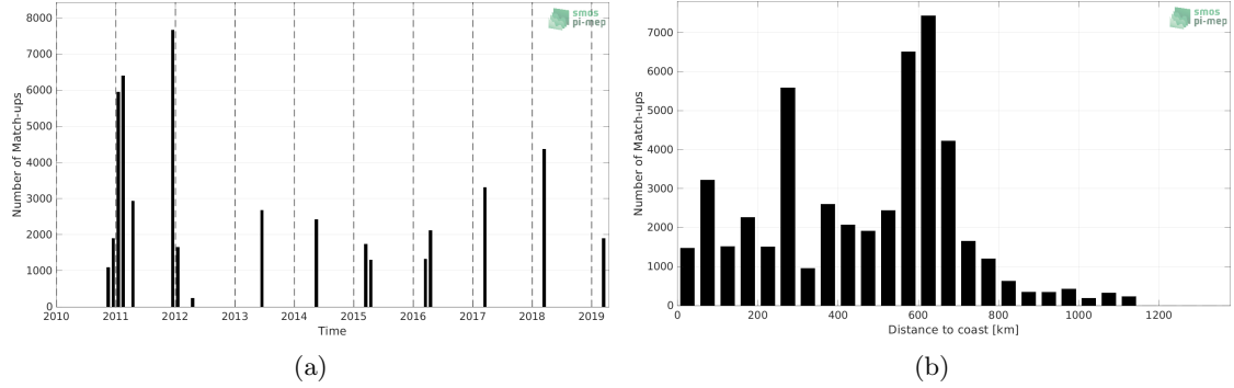
Figure 1: Number of match-ups between TSG (GOSUD-Research-vessel) and SMOS SSS L4 v1 - Monthly (CMEMS-CNR) SSS as a function of time (a) and as function of the distance to coast (b) over the Congo river plume Pi-MEP region and for the full satellite product period.
