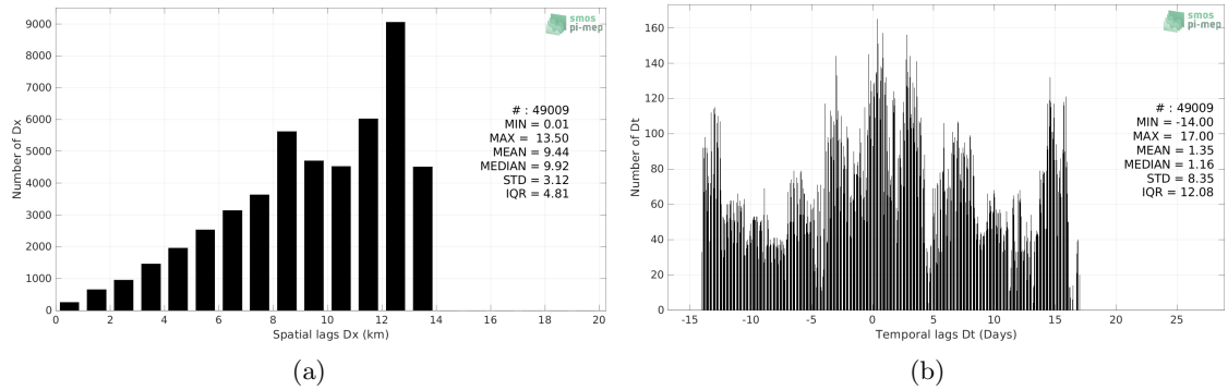
Figure 5: Histograms of the spatial (a) and temporal (b) lags between the location/time of the TSG (GOSUD-Research-vessel) measurement and the date of the corresponding SMOS SSS L4 v1 - Monthly (CMEMS-CNR) SSS pixel.
