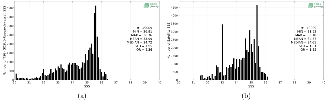
Figure 2: Histograms of SSS from TSG (GOSUD-Research-vessel) (a) and SMOS SSS L4 v1 - Monthly (CMEMS-CNR) (b) considering all match-up pairs per bins of 0.1 over the Congo river plume Pi-MEP region and for the full satellite product period.
