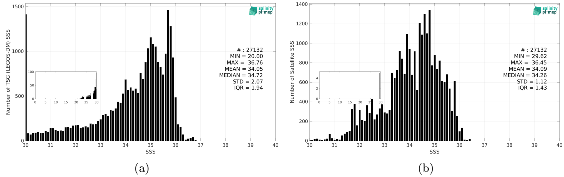
Figure 3: Histograms of SSS from TSG (LEGOS-DM) (a) and SMOS SSS L4 v1 - Daily (CMEMS-CNR) (b) considering all match-up pairs per bins of 0.1 over the Congo river plume Pi-MEP region and for the full satellite product period.
