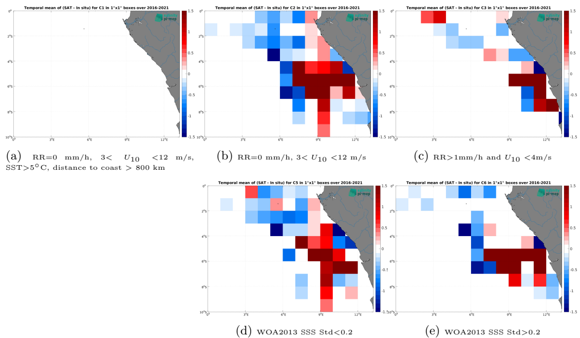
Figure 14: Temporal mean gridded over spatial boxes of size 1^\circ \times 1^\circ of \Delta SSS (SMOS SSS L4 v1 - Daily (CMEMS-CNR) - TSG (LEGOS-DM)) for 5 different subdatasets corresponding to:RR=0 mm/h, 3 < U_{10} < 12 m/s, SST>5°C, distance to coast > 800 km (a), RR=0 mm/h, 3 < U_{10} < 12 m/s (b), RR>1mm/h and U_{10} < 4 m/s (c), WOA2013 SSS Std<0.2 (d), WOA2013 SSS Std>0.2 (e).
