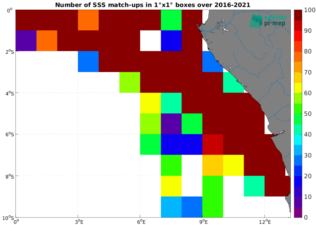
Figure 5: Number of SSS match-ups between TSG (LEGOS-DM) SSS and the SMOS SSS L4 v1 - Daily (CMEMS-CNR) SSS product for the Congo river plume Pi-MEP region over 1^\circ \times 1^\circ boxes and for the full satellite product period.
