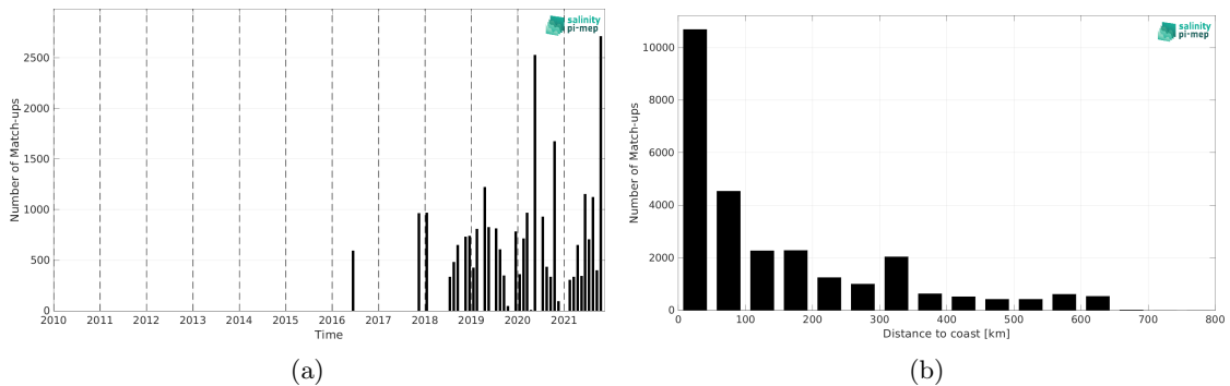
Figure 2: Number of match-ups between TSG (LEGOS-DM) and SMOS SSS L4 v1 - Daily (CMEMS-CNR) SSS as a function of time (a) and as function of the distance to coast (b) over the Congo river plume Pi-MEP region and for the full satellite product period.
