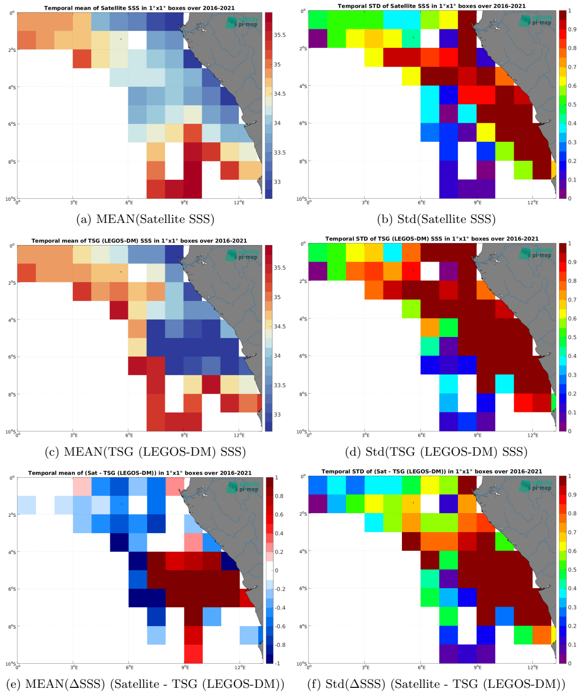
Figure 7: Temporal mean (left) and Std (right) of SSS from SMOS SSS L4 v1 - Daily (CMEMS-CNR) (top), TSG (LEGOS-DM) (middle), and of \Delta SSS (Satellite - TSG (LEGOS-DM)). Only match-up pairs are used to generate these maps.
