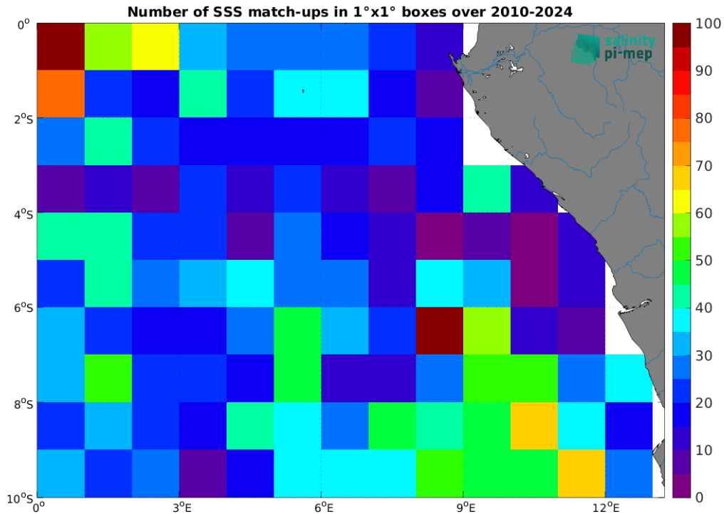
Figure 5: Number of SSS match-ups between Argo SSS and the SMOS SSS L4 v1 - Daily (CMEMS-CNR) SSS product for the Congo river plume Pi-MEP region over 1^\circ \times 1^\circ boxes and for the full satellite product period.
