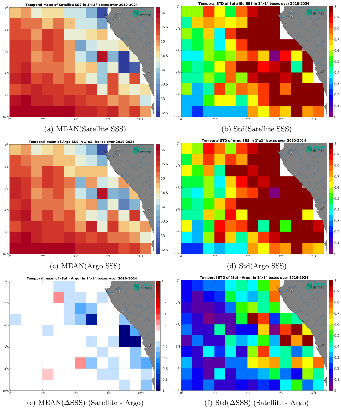
Figure 7: Temporal mean (left) and Std (right) of SSS from SMOS SSS L4 v1 - Daily (CMEMS-CNR) (top), Argo (middle), and of \Delta SSS (Satellite - Argo). Only match-up pairs are used to generate these maps.
