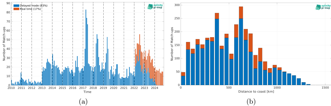
Figure 2: Number of match-ups between Argo and SMOS SSS L4 v1 - Daily (CMEMS-CNR) SSS as a function of time (a) and as function of the distance to coast (b) over the Congo river plume Pi-MEP region and for the full satellite product period.
