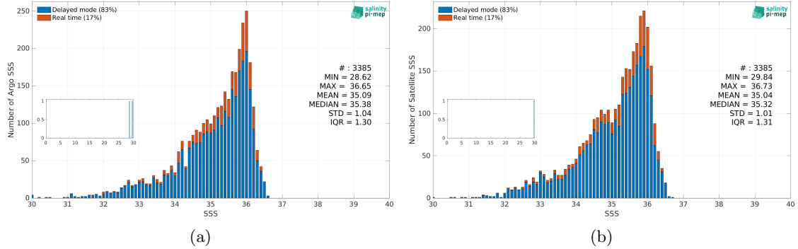
Figure 3: Histograms of SSS from Argo (a) and SMOS SSS L4 v1 - Daily (CMEMS-CNR) (b) considering all match-up pairs per bins of 0.1 over the Congo river plume Pi-MEP region and for the full satellite product period.
