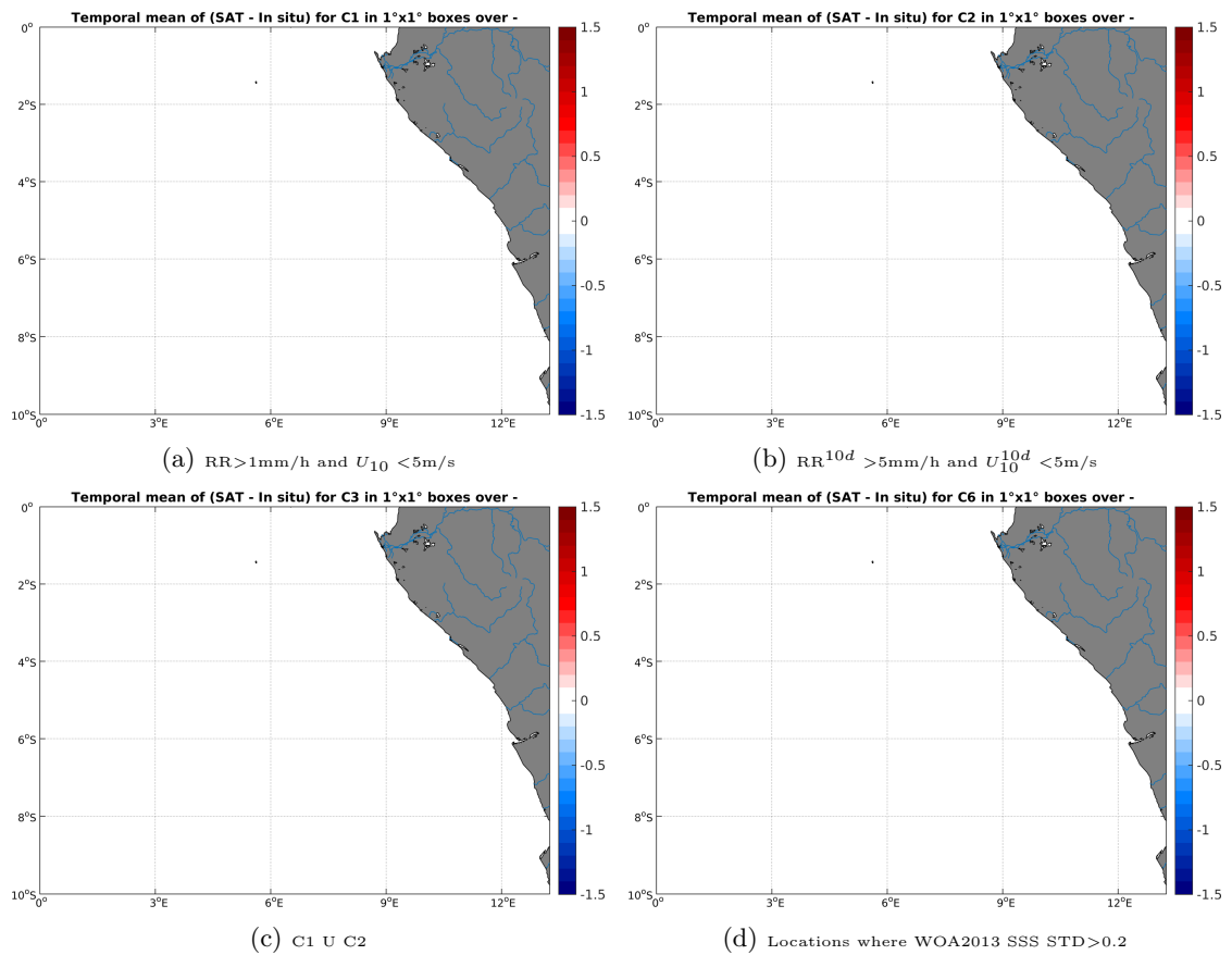
Figure 12: Temporal mean gridded over spatial boxes of size 1^\circ \times 1^\circ of \Delta SSS (SMOS-L4-CATDS-CECOS-IFREMER-V2-WEEKLY-0.5DEG - TSG-SAMOS) for 4 different subdatasets corresponding to:RR >1 mm/h and U_{10} < 5 m/s (a), RR ^{10d} > 5 mm/h and U_{10}^{10d} < 5 m/s (b), C1 U C2 (c),Locations where WOA2013 SSS STD >0.2 (d).
