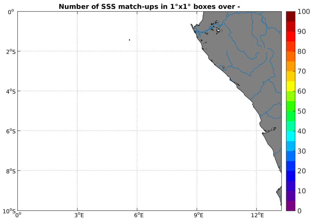
Figure 4: Number of SSS match-ups between TSG-SAMOS SSS and the SMOS-L4-CATDS-CECOS-IFREMER-V2-WEEKLY-0.5DEG SSS product for the Congo river plume Pi-MEP region over 1°x1° boxes and for the full satellite product period.
