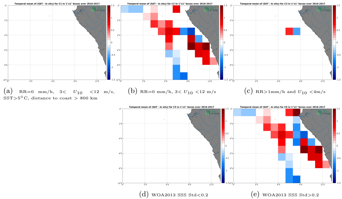
Figure 12: Temporal mean gridded over spatial boxes of size 1^\circ \times 1^\circ of \Delta SSS (SMOS-L4-CATDS-CECOS-IFREMER-V2-WEEKLY-0.5DEG - TSG-LEGOS-DM) for 5 different subdatasets corresponding to:RR=0 mm/h, 3 < U_{10} < 12 m/s, SST > 5^\circ\text{C} , distance to coast > 800 km (a), RR=0 mm/h, 3 < U_{10} < 12 m/s (b), RR > 1 mm/h and U_{10} < 4 m/s (c), WOA2013 SSS Std < 0.2 (d), WOA2013 SSS Std > 0.2 (e).
