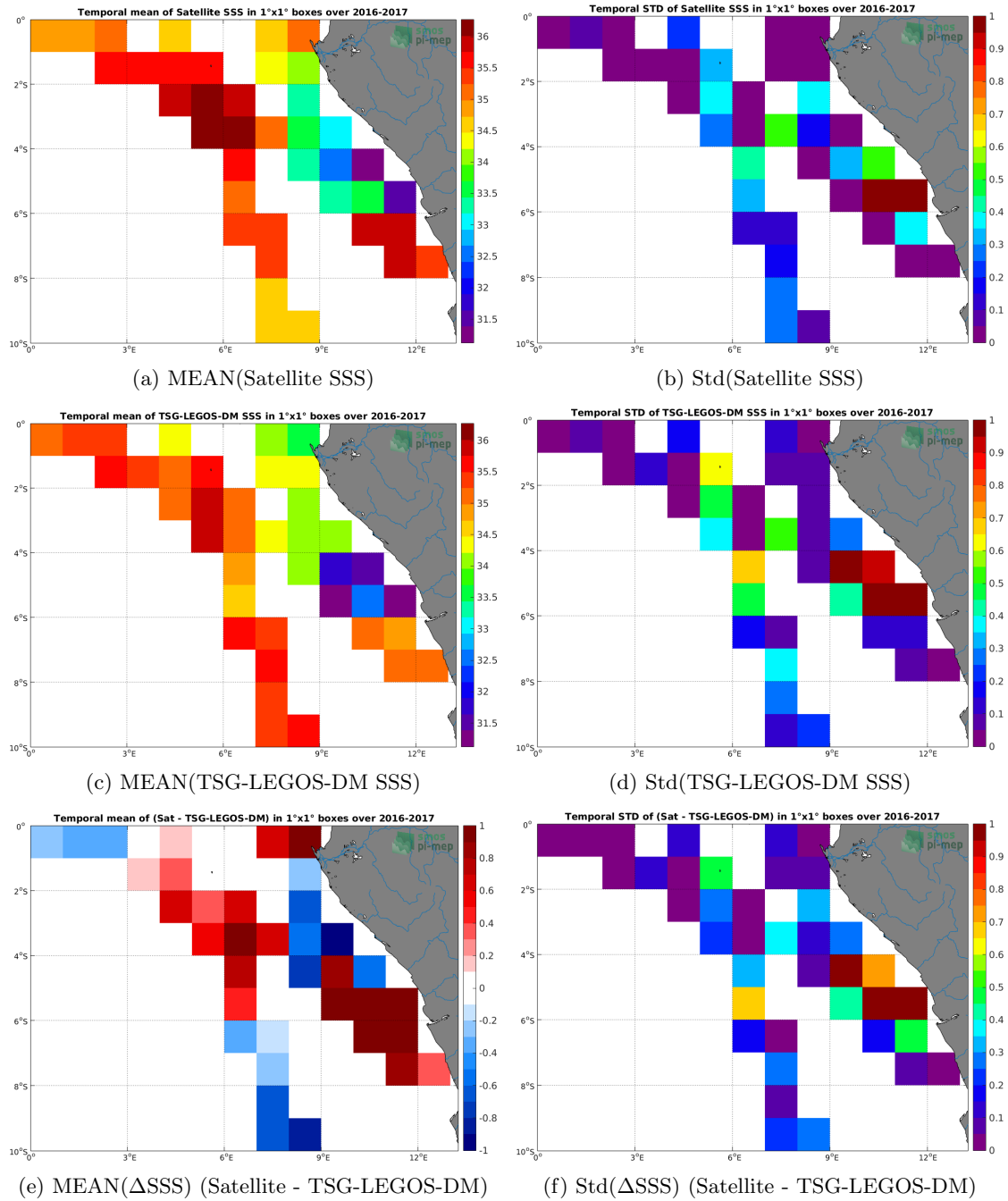
Figure 6: Temporal mean (left) and Std (right) of SSS from SMOS-L4-CATDS-CECOS-IFREMER-V2-WEEKLY-0.5DEG (top), TSG-LEGOS-DM (middle), and of \Delta SSS (Satellite - TSG-LEGOS-DM). Only match-up pairs are used to generate these maps.
