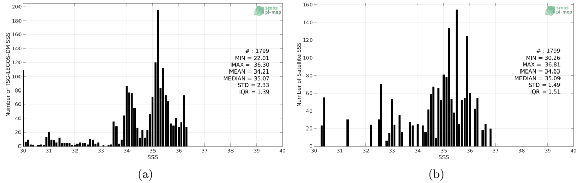
Figure 2: Histograms of SSS from TSG-LEGOS-DM (a) and SMOS-L4-CATDS-CECOS-IFREMER-V2-WEEKLY-0.5DEG (b) considering all match-up pairs per bins of 0.1 over the Congo river plume Pi-MEP region and for the full satellite product period.
