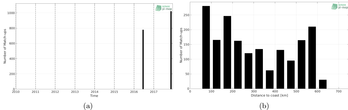
Figure 1: Number of match-ups between TSG-LEGOS-DM and SMOS-L4-CATDS-CECOS-IFREMER-V2-WEEKLY-0.5DEG SSS as a function of time (a) and as function of the distance to coast (b) over the Congo river plume Pi-MEP region and for the full satellite product period.
