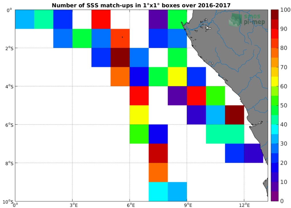
Figure 4: Number of SSS match-ups between TSG-LEGOS-DM SSS and the SMOS-L4-CATDS-CECOS-IFREMER-V2-WEEKLY-0.5DEG SSS product for the Congo river plume Pi-MEP region over 1^\circ \times 1^\circ boxes and for the full satellite product period.
