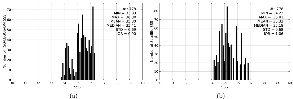
Figure 2: Histograms of SSS from TSG-LEGOS-DM (a) and SMOS-L4-CATDS-CECOS-IFREMER-V2-WEEKLY-0.5DEG (b) considering all match-up pairs per bins of 0.1 over the Congo river plume Pi-MEP region and for the full satellite product period.
