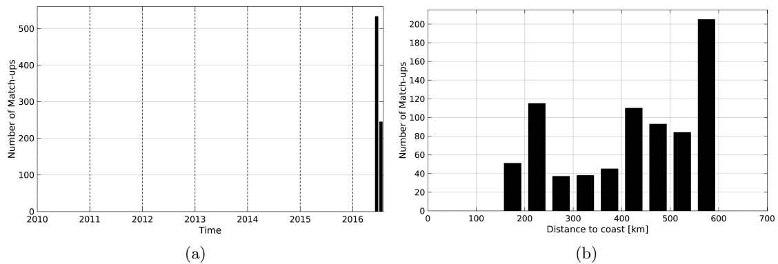
Figure 1: Number of match-ups between TSG-LEGOS-DM and SMOS-L4-CATDS-CECOS-IFREMER-V2-WEEKLY-0.5DEG SSS as a function of time (a) and as function of the distance to coast (b) over the Congo river plume Pi-MEP region and for the full satellite product period.
